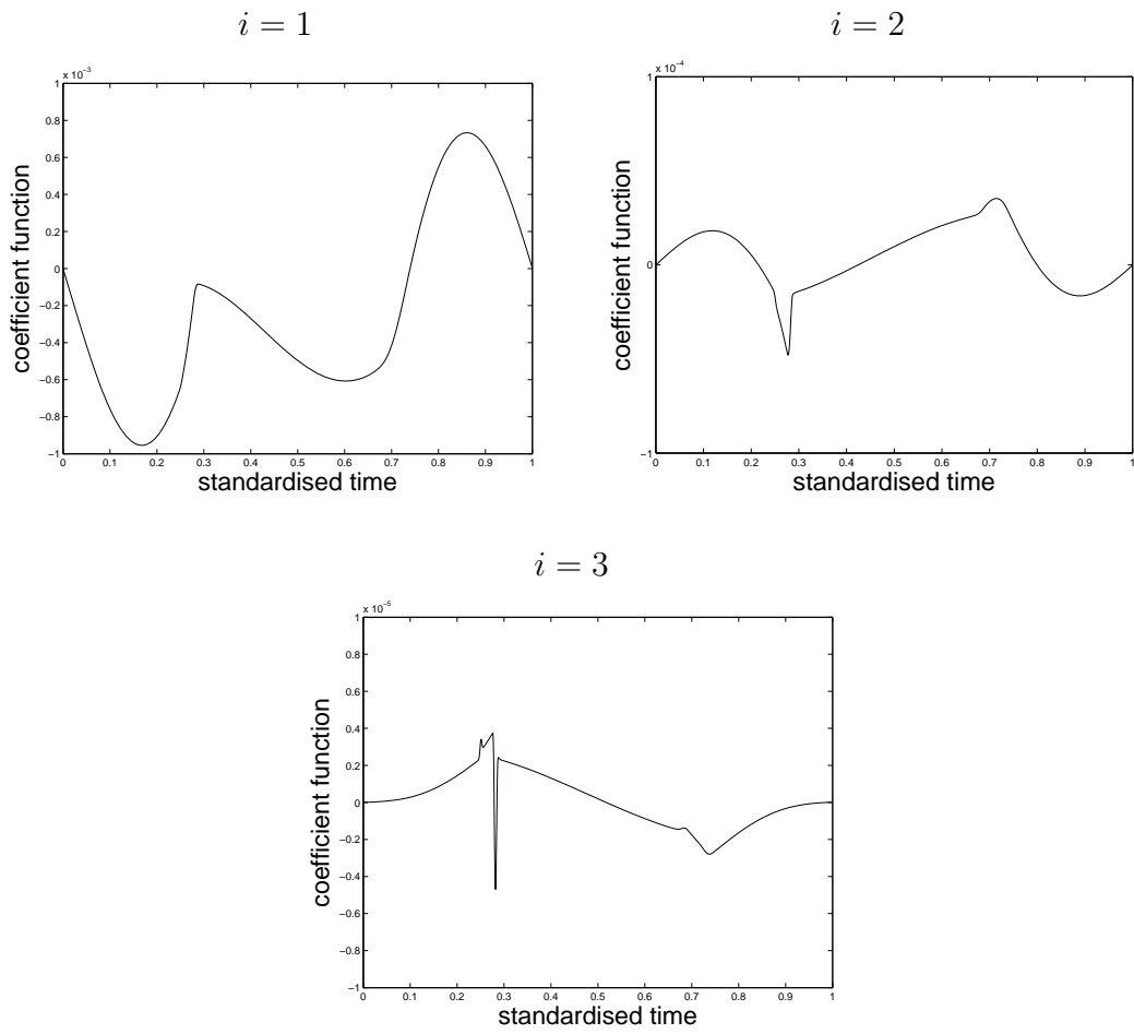
Figure 5: Coefficient functions v_i of gPC expansion for u_1 .
