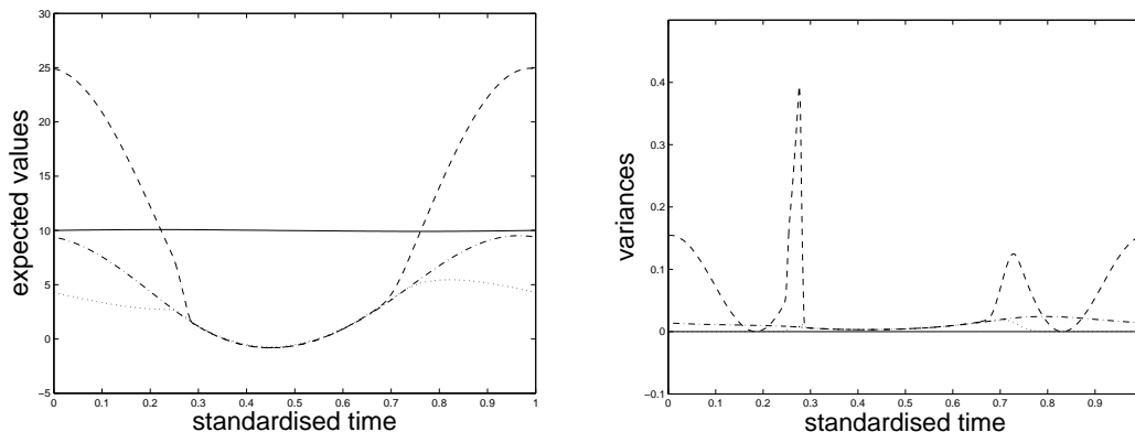
Figure 4: Expected values (left) and variances (right) of all components obtained by gPC simulation of Colpitt oscillator ( u_1 : —, u_2 : - - -, u_3 : - · - ·, u_4 : · · ·).
