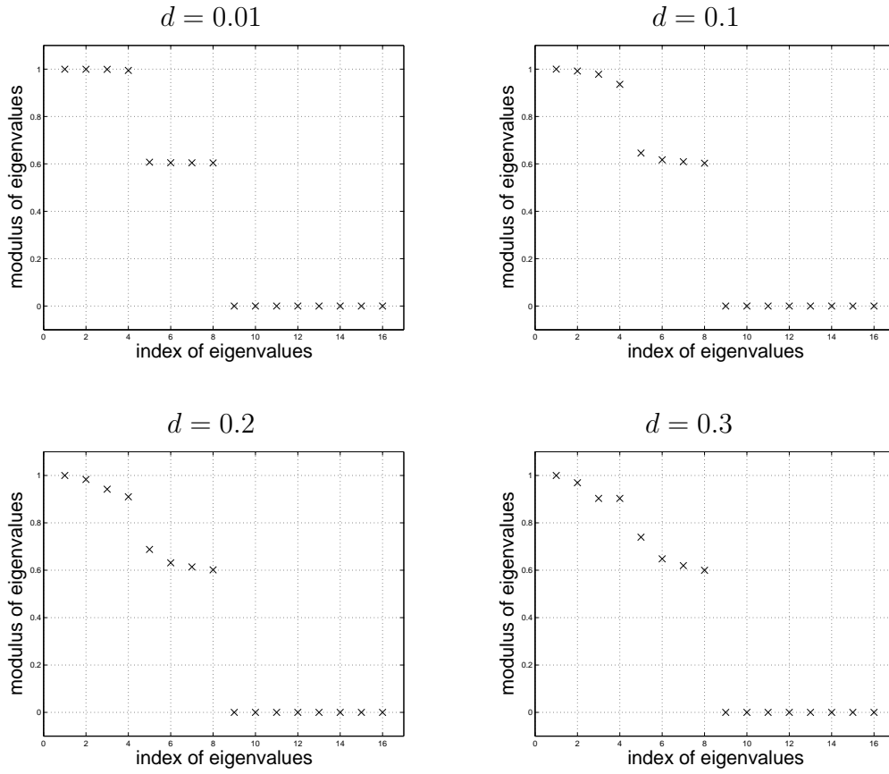
Figure 8: Eigenvalues of monodromy matrix for gPC system corresponding to Colpitt oscillator. Different magnitudes d of the uncertainty are applied in (32).
