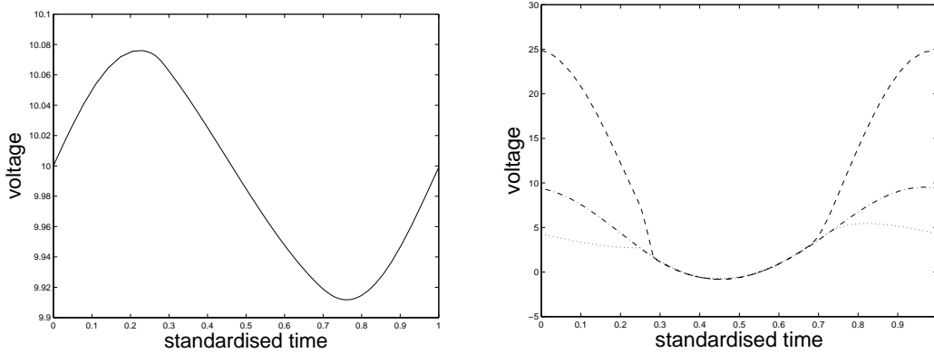
Figure 3: Periodic solution of Colpitt oscillator obtained via a phase condition ( u_1 : —, u_2 : - - -, u_3 : - · - · -, u_4 : ···).
