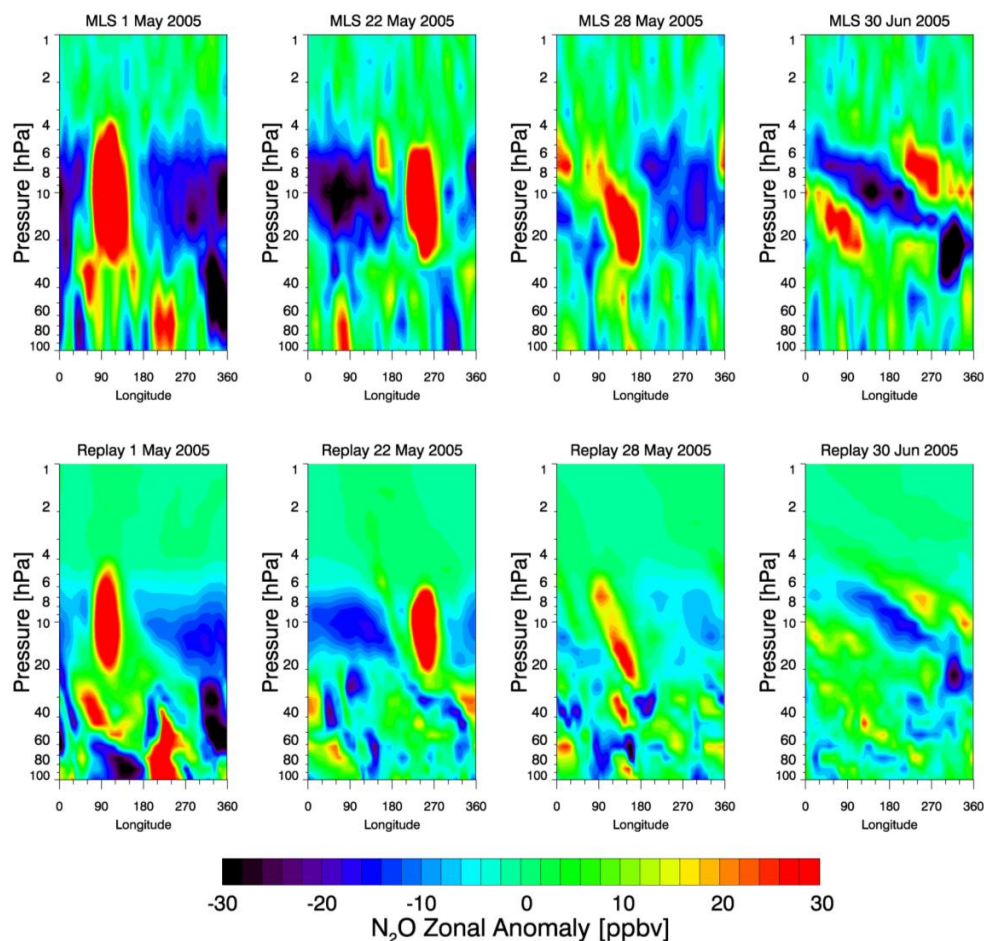
Fig. 13. Longitude vs. pressure cross-sections at 74° N latitude of MLS and Replay N 2 O (deviation from zonal mean) for 1, 22, and 28 May and 30 June 2005. Red (blue) indicates high (low) N 2 O zonal anomaly.
