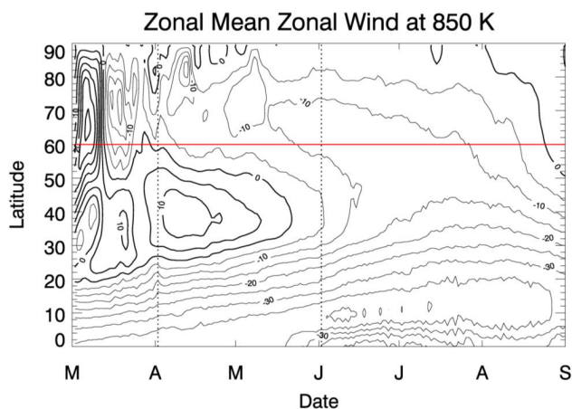
Fig. 1. Zonal mean zonal wind at 850 K potential temperature for March–August 2005. Vertical dotted lines indicate transitions between the three phases of the FrIAC (see text for details), while the red line marks 60° N latitude.
