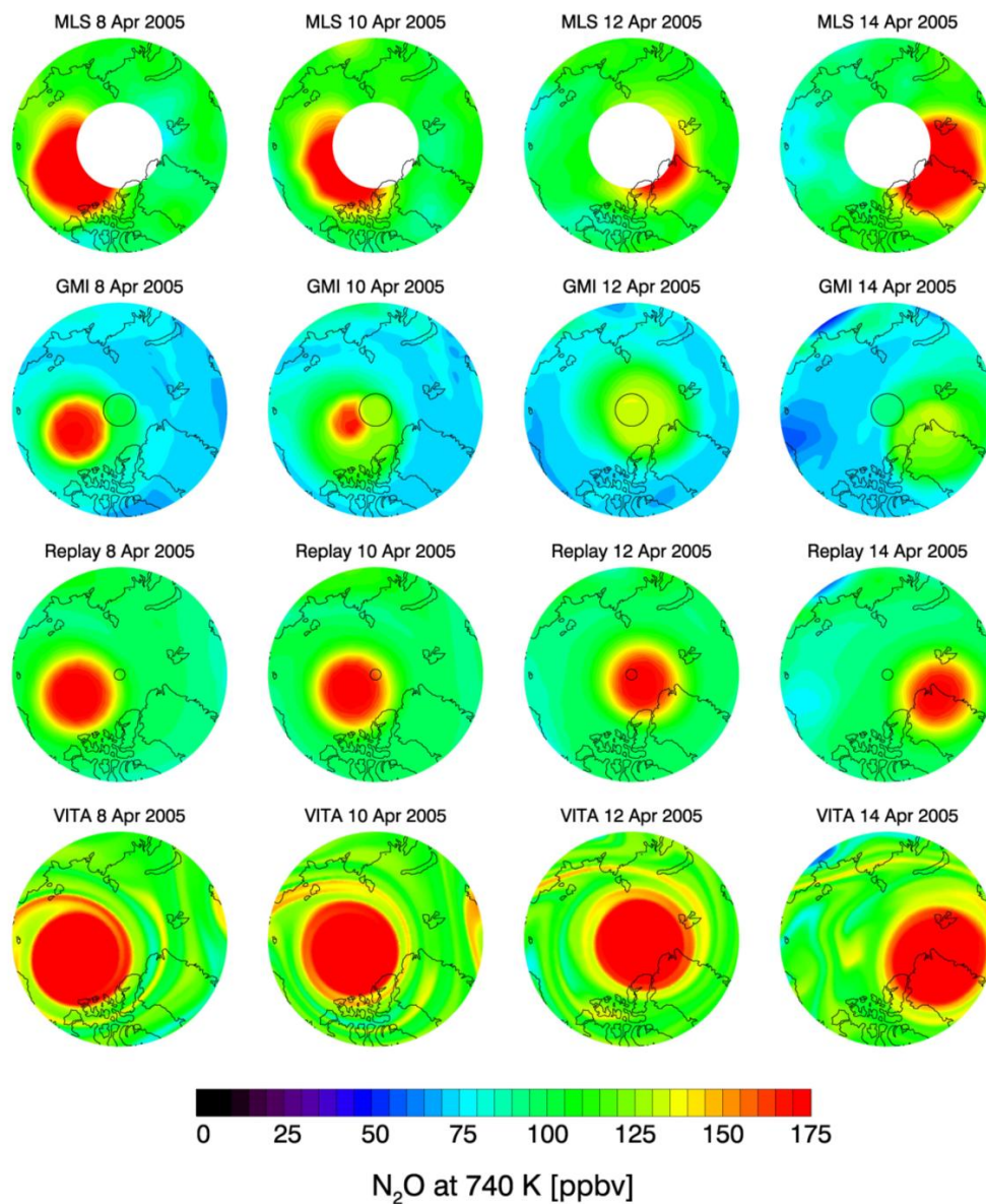
Fig. 10. MLS \text{N}_2\text{O} mixing ratio from 70\text{--}90^\circ\text{N} at 740 K potential temperature for 8, 10, 12, and 14 April 2005 along with simulations from GMI, Replay, and VITA. Red (blue) indicates high (low) \text{N}_2\text{O} values. Black circles indicate the extent of the polar mixing cap in the GMI and Replay simulations.
