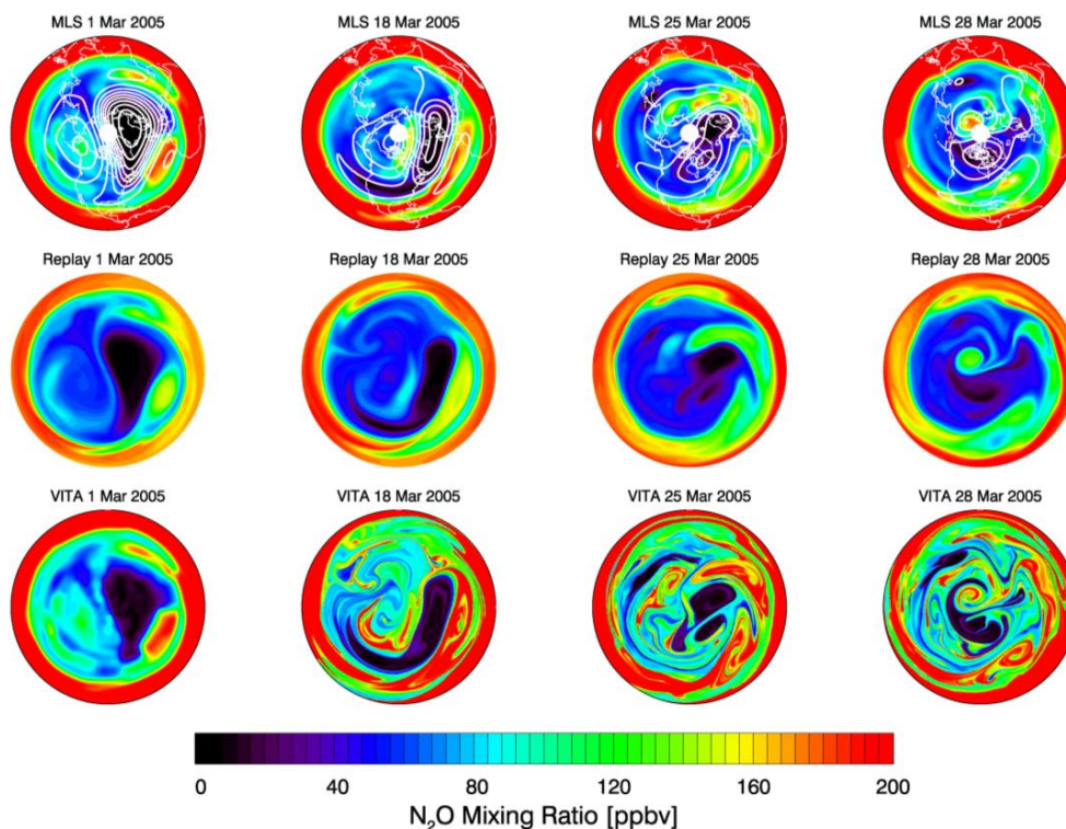
Fig. 4. Northern Hemisphere EOS Aura MLS \text{N}_2\text{O} mixing ratio at 850 K for 1, 18, 25, and 28 March 2005 overlaid with contours of 10 hPa geopotential height at 250-m intervals (first row). Red (blue) indicates high (low) \text{N}_2\text{O} values. Replay \text{N}_2\text{O} simulations for the same days (second row). VITA \text{N}_2\text{O} simulations initialized on 1 March 2005 (third row).
