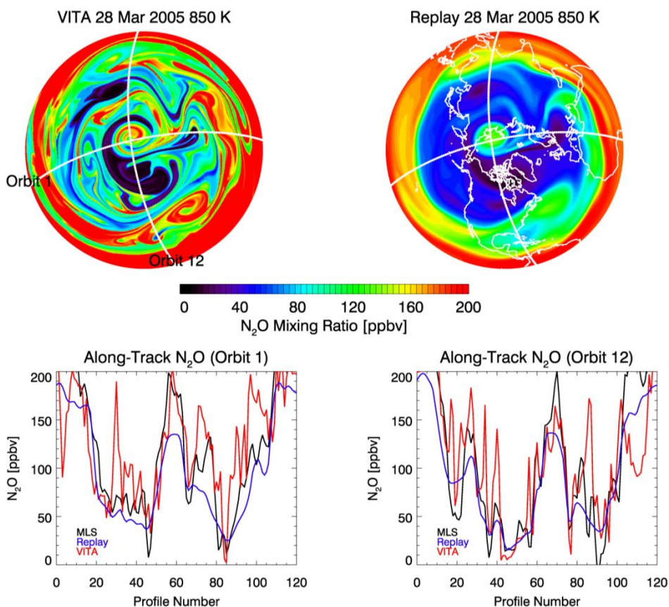
Fig. 5. Top row: Northern Hemisphere VITA (left) and Replay (right) \text{N}_2\text{O} at 850 K on 28 March 2005. Red (blue) indicates high (low) \text{N}_2\text{O} values. Overlaid are two EOS Aura MLS orbit tracks for this day. Second row: MLS (black), Replay (blue), and VITA (red) \text{N}_2\text{O} at 850 K along the selected orbit tracks. The profiles start at the locations of the orbit labels in the upper left panel. Replay and VITA data are interpolated linearly in space and time to the MLS data points.
