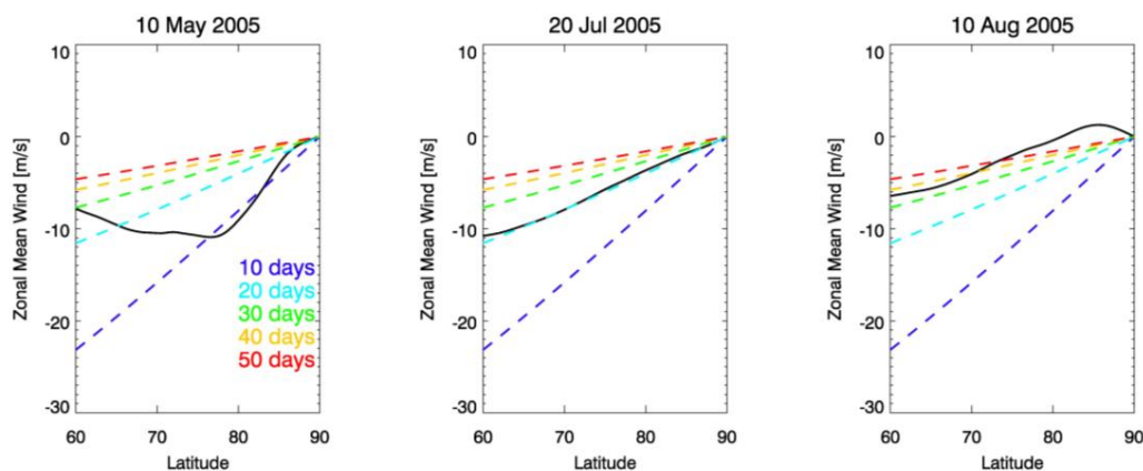
Fig. 12. Zonal mean zonal wind (black line) as a function of latitude at 850 K for 10 May, 20 July, and 10 August 2005. Color curves indicate the winds necessary for solid-body rotation with periods of 10 (blue), 20 (cyan), 30 (green), 40 (yellow), and 50 (red) days.
