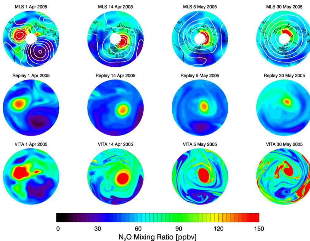
Fig. 9. MLS N 2 O mixing ratio at 850 K from 50–90° N for 1 and 14 April and for 5 and 30 May 2005 overlaid with contours of 10 hPa geopotential height at 100-m intervals (first row). Red (blue) indicates high (low) N 2 O values. Replay N 2 O simulations for the same days (second row). VITA N 2 O simulations initialized on 1 April 2005 (third row).
