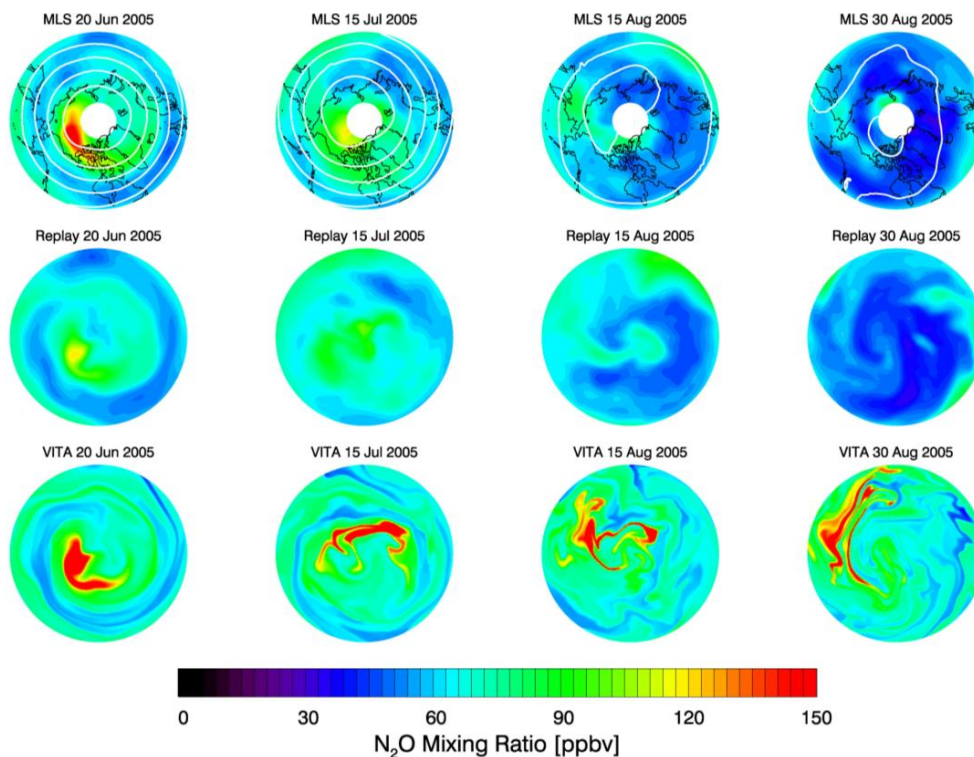
Fig. 14. MLS \text{N}_2\text{O} mixing ratio at 850 K from 50–90° N for 20 June, 15 July, and 15 and 30 August 2005 overlaid with contours of 10 hPa geopotential height at 100-m intervals (first row). Red (blue) indicates high (low) \text{N}_2\text{O} values. Replay \text{N}_2\text{O} simulations for the same days (second row). VITA \text{N}_2\text{O} simulations initialized on 1 June 2005 (third row).
