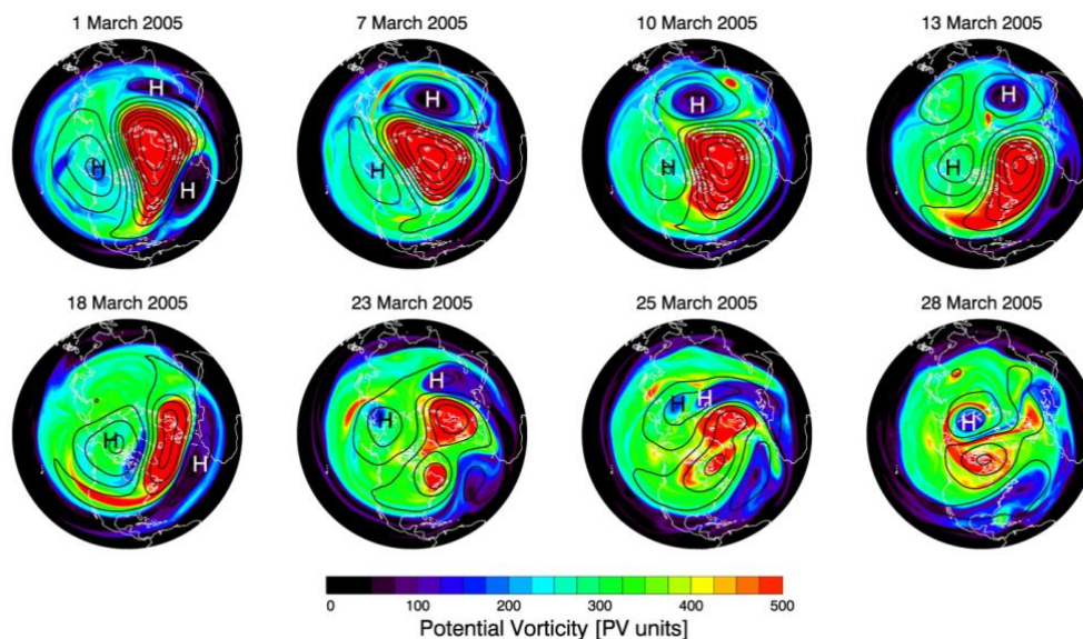
Fig. 2. Northern Hemisphere Ertel potential vorticity at 850 K potential temperature for 1, 7, 10, 13, 18, 23, 25, and 28 March 2005. PV units are used, where 1 \text{ PVU} = 1.0 \times 10^{-6} \text{ m}^2 \text{ s}^{-1} \text{ K kg}^{-1} . Red (blue) indicates high (low) values of PV. Black lines indicate 10 hPa geopotential height at 250-m contour intervals. The black “H” marks the location of the Aleutian anticyclone and the white “H”s mark the locations of other anticyclones.
