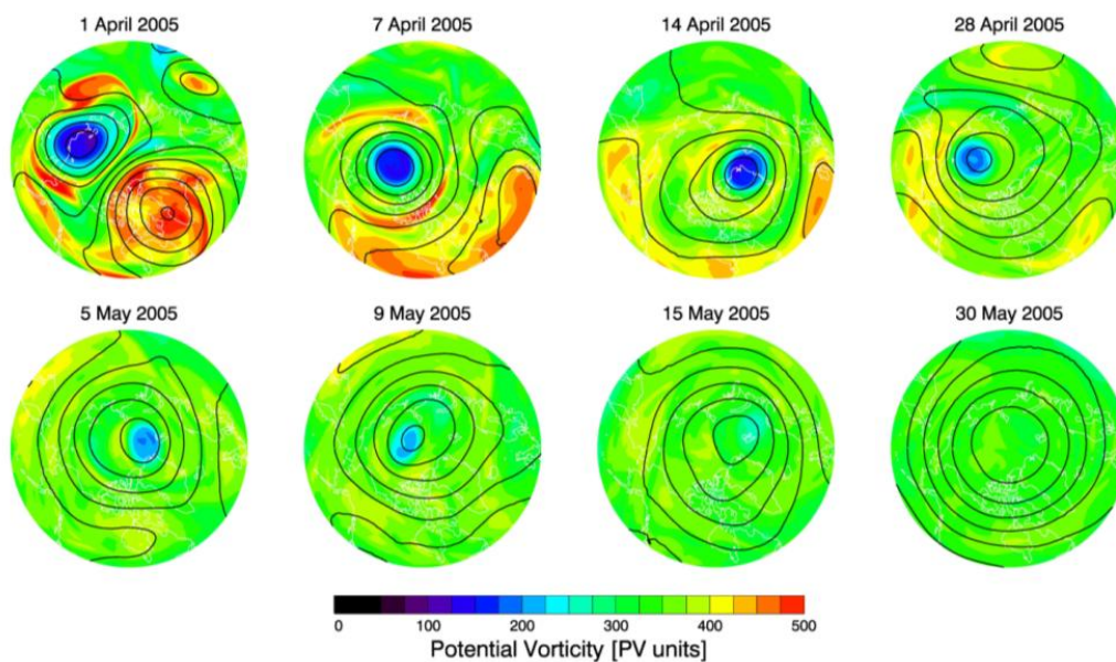
Fig. 8. Ertel potential vorticity at 850 K potential temperature from 50–90° N for 1, 7, 14, and 28 April and 5, 9, 15, and 30 May 2005. Red (blue) indicates high (low) PV values. Black lines indicate 10 hPa geopotential height at 100-m contour intervals.
