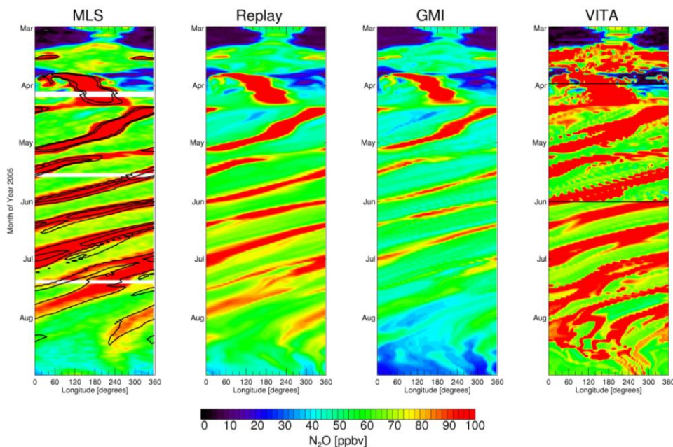
Fig. 16. Longitude vs. time Hovmöller plots of \text{N}_2\text{O} at 850 K, 78^\circ N for MLS, Replay, GMI, and VITA from March to September 2005. Red (blue) indicates high (low) \text{N}_2\text{O} values. The black contours on the MLS plot are the 75 and 100 ppbv contours of the Replay simulation, for direct comparison with MLS. White regions on the MLS plot indicate no data available during that time period. The VITA contours are produced from a composite of three runs of the model, initialized with MLS \text{N}_2\text{O} on 1 March, 1 April, and 1 June, as indicated by the horizontal black lines.
