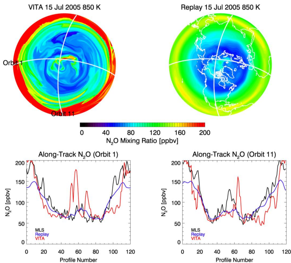
Fig. 15. Top row: Northern Hemisphere VITA (left) and Replay (right) N 2 O at 850 K on 15 July 2005. Red (blue) indicates high (low) N 2 O values. Overlaid are two EOS Aura MLS orbit tracks for this day. Second row: MLS, Replay, and VITA N 2 O at 850 K along the selected orbit tracks. The profiles start at the locations of the orbit labels in the upper left panel. Replay and VITA data are interpolated linearly in space and time to the MLS data points.
