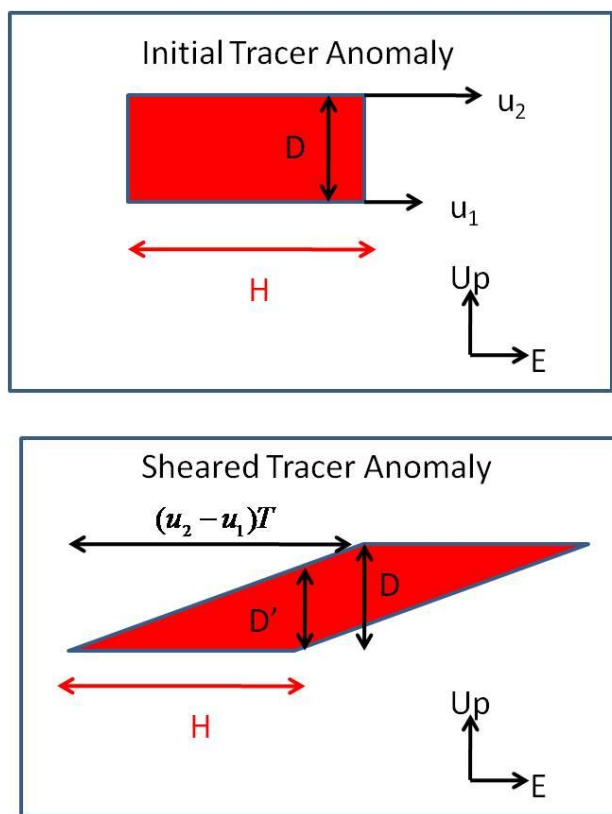
Fig. 17. Schematic diagram of an idealized passive tracer anomaly subject to linear vertical shear of the (steady) zonal wind (east (E) is to the right and U_p points vertically upward in both figures). The tracer anomaly initially has a height scale D and width (in the east-west direction) H . The vertical shear is indicated by a difference in zonal wind at the bottom of the anomaly ( u_1 ) and at the top of the anomaly ( u_2 ). The top panel shows the initial tracer anomaly and the bottom panel shows the sheared tracer anomaly at time T after the top of the anomaly has completely passed the base of the anomaly. The vertical thickness of the anomaly is now D' .
