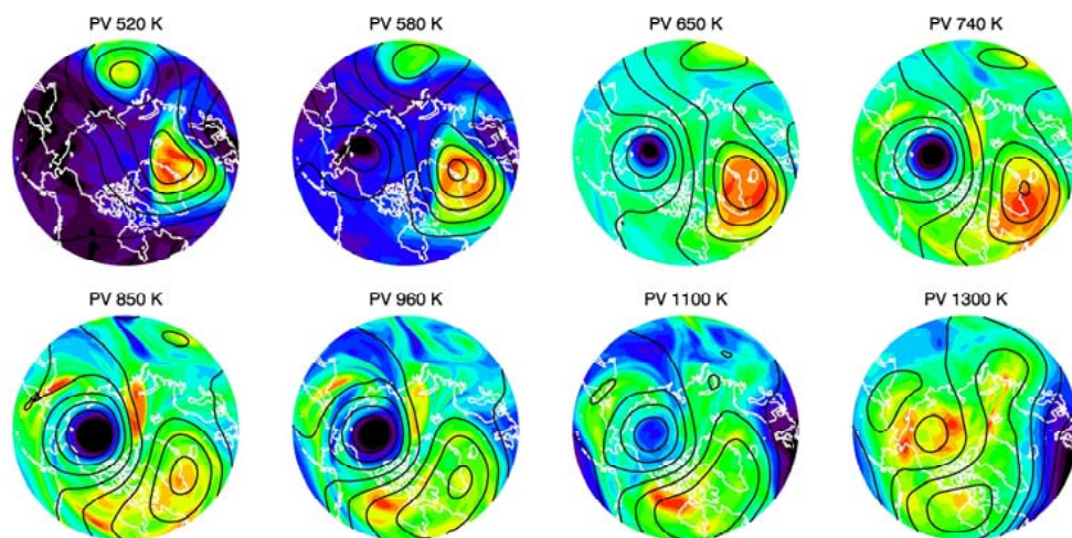
Fig. 3. Ertel potential vorticity at eight potential temperature levels (520, 580, 650, 740, 850, 960, 1100, and 1300 K) from 50–90° N on 4 April 2005 (Greenwich Meridian is on the right side). Colors are scaled to the range of PV values for the given level, with red (blue) indicating high (low) PV. Black lines show 10 hPa geopotential height at 100-m contour intervals.
