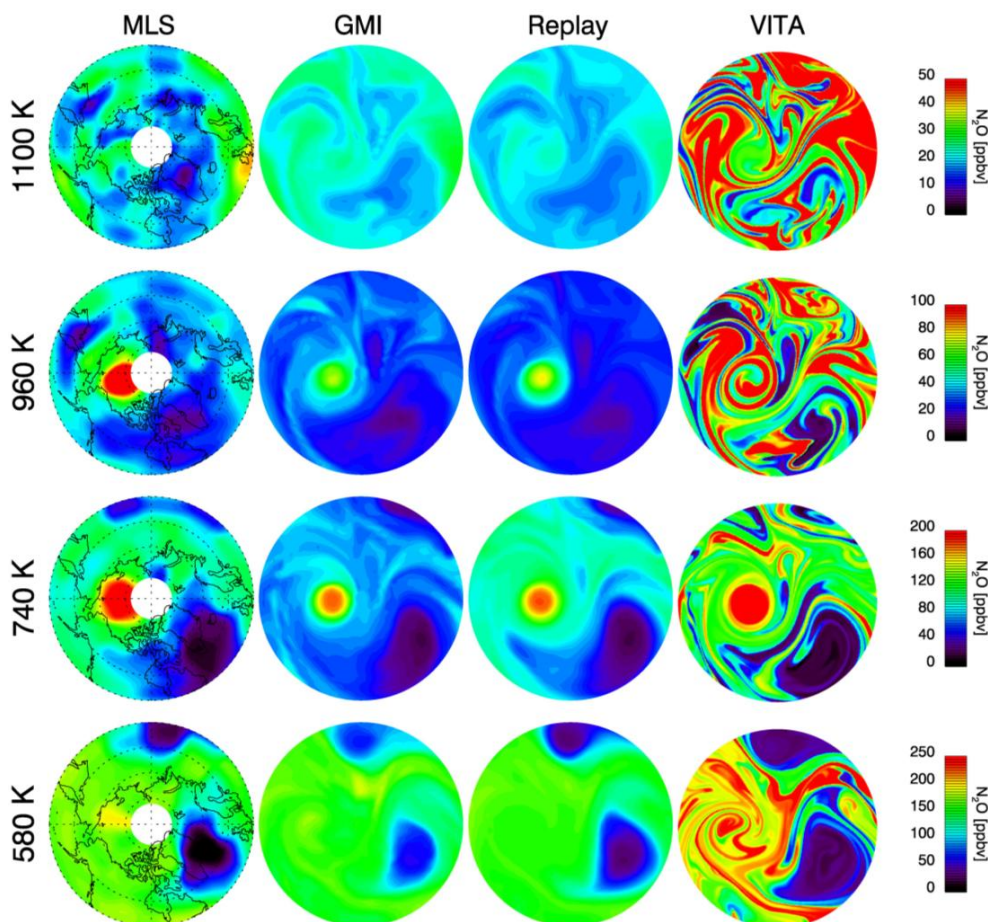
Fig. 7. MLS \text{N}_2\text{O} (first column) from 50\text{--}90^\circ\text{N} at several potential temperature levels (rows correspond to 1100, 960, 740, and 580 K) for 4 April 2005 along with simulations from GMI (second column), Replay (third column), and VITA (fourth column). Red (blue) indicates high (low) \text{N}_2\text{O} values.
