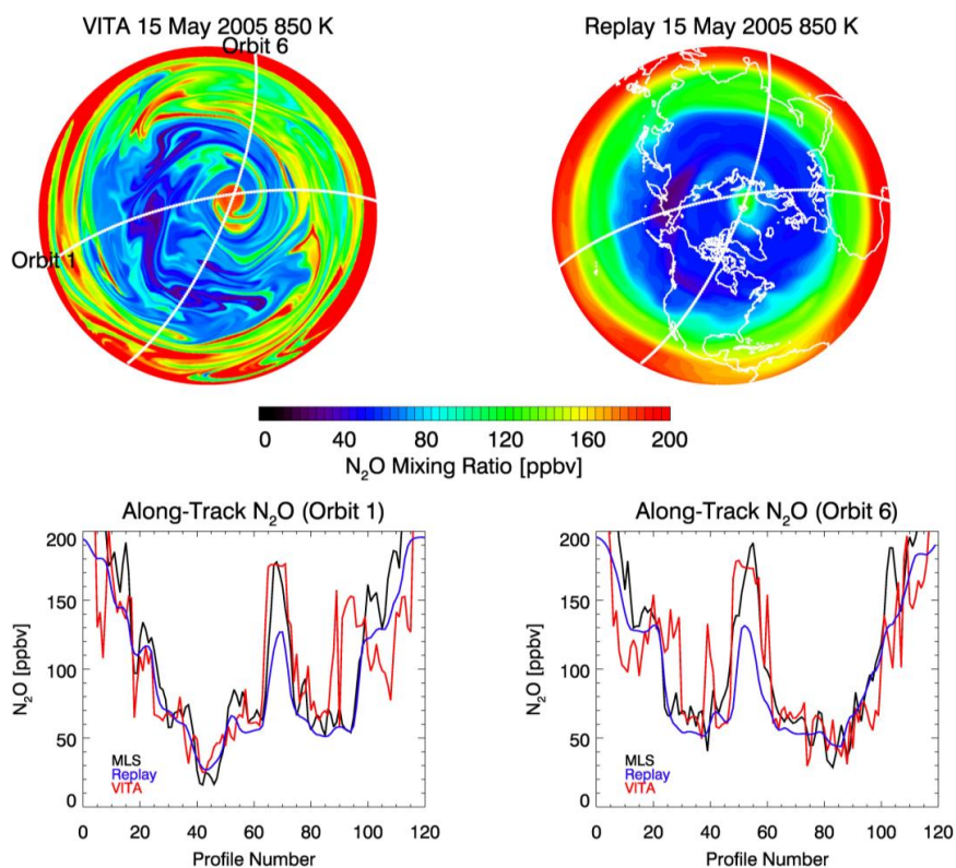
Fig. 11. Top row: Northern Hemisphere VITA (left) and Replay (right) \text{N}_2\text{O} at 850 K on 15 May 2005. Red (blue) indicates high (low) \text{N}_2\text{O} values. Overlaid are two EOS Aura MLS orbit tracks for this day. Second row: MLS, Replay, and VITA \text{N}_2\text{O} at 850 K along the selected orbit tracks. The profiles start at the locations of the orbit labels in the upper left panel. Replay and VITA data are interpolated linearly in space and time to the MLS data points.
