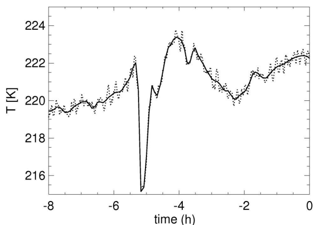
Fig. 4. Solid black line: temperature along a COSMO-7-based LAGRANTO trajectory in about 9 km altitude (close to cloud “L”). Dotted line: same trajectory with superimposed small-scale temperature fluctuations (dT/dt)_{ss} (random superposition). The cooling rate spectrum has been determined from the variance ( 0.2 \text{ K}^2 ) and frequencies of (dT/dt)_{ss} with wavelengths smaller than 30 km (see text) in agreement with the vertical wind measurements made during the SUCCESS campaign (see Hoyle et al., 2005).
