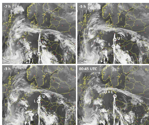
Fig. A1. Cloud images from the Meteosat satellite at four different times (Eumetsat, 2012). White lines: projections of the trajectories ending in the upper “U” and lower “L” cloud at 00:45 UTC. White circles: respective positions of air parcels 7 h, 5 h and 3 h upstream.
