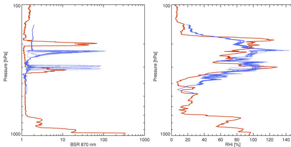
Fig. 6. Ensemble of 20 microphysical column model runs (blue) with superimposed small-scale fluctuations compared with the measurements (red). The left panel shows BSR_{870} and the right RH_{ice} .
