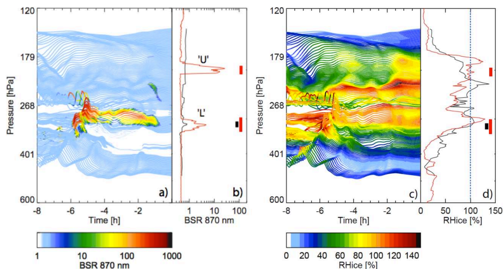
Fig. 3. Results from the microphysical column model ZOMM on LAGRANTO trajectories driven by COSMO-7 meteorological fields (5 min resolution) compared to measurements of backscatter ratio ( BSR ) at 870 nm wavelength ( a , b ) and relative humidity ( RH_{ice} ) with respect to ice ( c , d ). ( a , c ) Colour-coded: modelled BSR and RH_{ice} . ( b , d ) Red curves: BSR and RH_{ice} profiles measured by COBALD and CFH, respectively; black curves: model results at t=0 above Lindenberg (right edge of ( a ) and ( c )). The model produces both clouds (“U” and “L”) a few hours upstream of the measurement, but due to too rapid sedimentation fails to maintain them until the measurement time. Red and black bars in ( b ) and ( d ) indicate the altitude ranges of the measured clouds and modelled cloud remnants, respectively.
