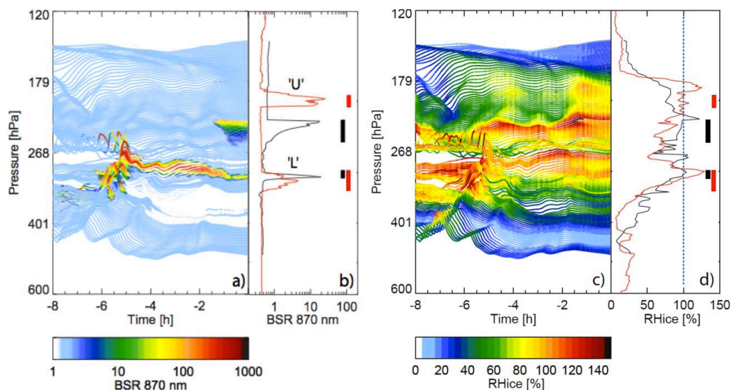
Fig. 5. Results from microphysical column model driven by COSMO-7-based LAGRANTO trajectories with superimposed small-scale temperature fluctuations (dT/dt)_{ss} compared to measurements of backscatter ratio ( BSR ) at 870 nm wavelength ( a , b ) and relative humidity ( RH_{ice} ) with respect to ice ( c , d ). ( a , c ) Colour-coded: modelled BSR and RH_{ice} . ( b , d ) Red curves: BSR and RH_{ice} profiles measured by COBALD and CFH, respectively; black curves: model results at t=0 above Lindenberg (right edge of ( a ) and ( c )). The model produces both clouds (“U” and “L”) a few hours upstream of the measurement, and due to (dT/dt)_{ss} forms sufficiently small ice particles, which survive until the measurement time. Red and black bars in ( b ) and ( d ) indicate the altitude ranges of the measured and modelled clouds, respectively.
