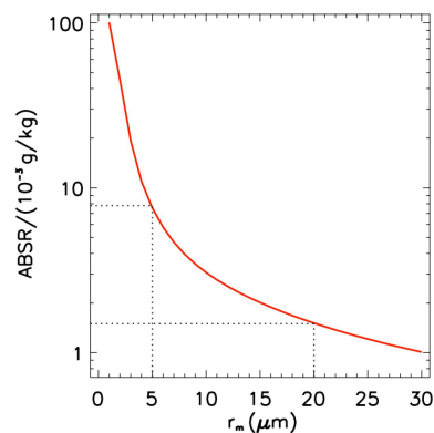
Fig. B1. Red curve: Simulated aerosol backscatter ratio ( ABSR ) at 870 nm wavelength per 10^{-3} \text{ g kg}^{-1} condensed as ice particles in a lognormal size distribution in dependence of the mode radius ( r_m ). The assumed conditions are a lognormal distribution width \sigma = 1.4 , a refractive index of 1.31 (for ice), and an aspect ratio A = 0.75 for prolate spheroids as proxy for the ice particle asphericity. ABSR for IWC other than 10^{-3} \text{ g kg}^{-1} are obtained by appropriate scaling of the ordinate. Black dotted lines: typical range of r_m in high thin cirrus clouds (which formed in situ, e.g. by orographically forced upwelling), resulting in an overall uncertainty in BSR of a factor of \sim 4 .
