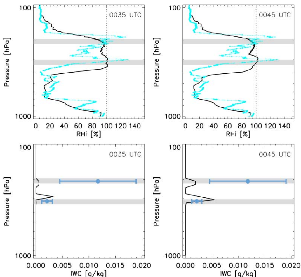
Fig. 2. RH_{ice} and IWC profiles of COSMO-7 forecast data (black lines) above Lindenberg on 6 November 2008. Left: sounding of lower cloud at 00:35 UTC. Right: sounding of upper cloud at 00:45 UTC. Cyan line: RH_{ice} profile measured by CFH. Grey horizontal bars: altitude ranges of the detected clouds. Blue bars in the lower two panels: IWC estimated from COBALD data as explained in Appendix A.
