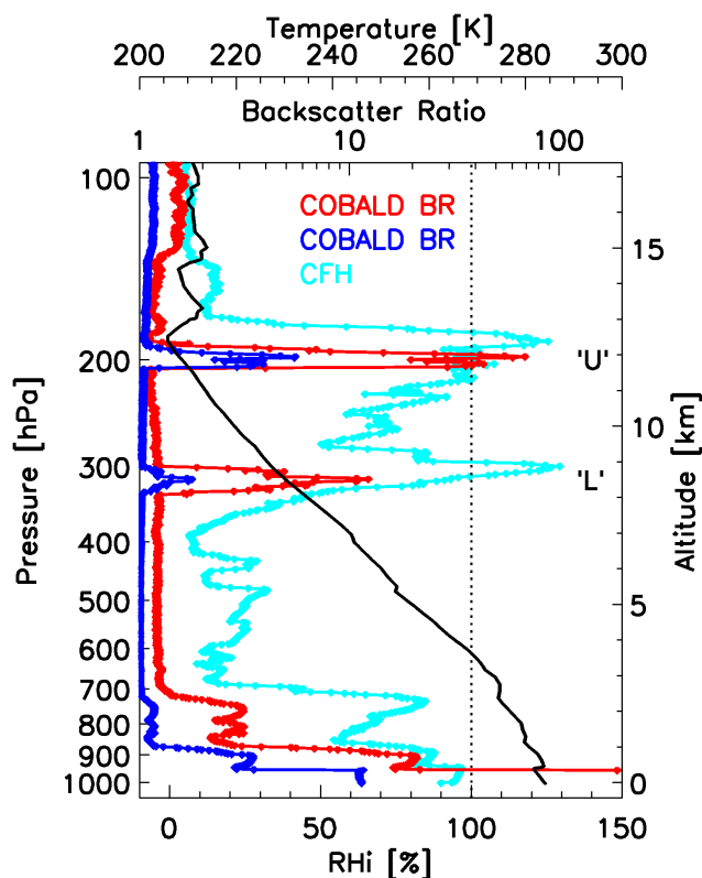
Fig. 1. Profile of balloon sounding on 6 November 2008 above Lindenberg, Germany. Blue and red lines: backscatter ratios ( BSR ) at 455 nm and 870 nm wavelength, respectively, measured by COBALD. Cyan line: relative humidity with respect to ice ( RH_{\text{ice}} ) obtained from the CFH frost point measurement. Quantities shown as function of barometric pressure and GPS-measured geometric altitude. The upper and lower cirrus clouds are termed ‘‘U’’ and ‘‘L’’, respectively.
