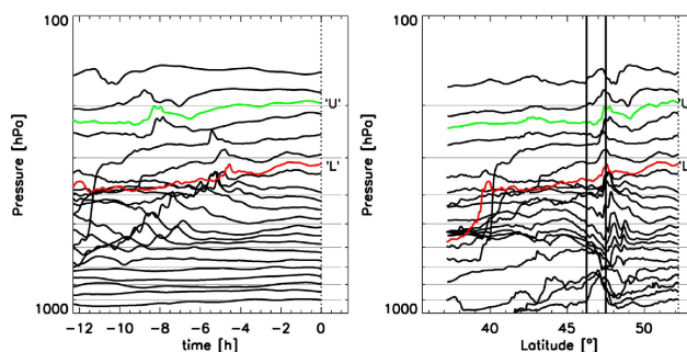
Fig. A2. Field of COSMO-7-based LAGRANTO trajectories highlighting the two trajectories ending in the lower cloud “L” (red) and upper cloud “U” (green). Left panel: trajectory pressure vs. time. Right panel: trajectory pressure vs. latitude. Waves are caused by the main chain of the Alps located around 47° N (indicated by vertical lines).
