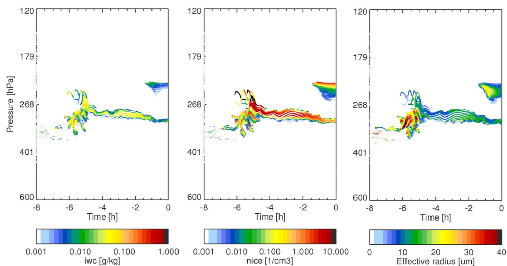
Fig. B2. Microphysical column model results for the case with superimposed small-scale temperature fluctuations showing parameters in addition to those shown in Fig. 5. Left panel: ice water content, IWC . Centre panel: ice number density, n_{ice} . Right panel: effective radius of the ice crystals, r_{eff} .
