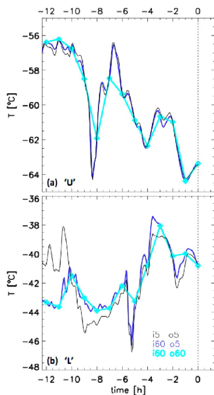
Fig. C1. Examples of backward trajectories for (a) the upper cloud “U”, (b) lower cloud “L”. Black curves: based on COSMO-7 fields with 5-min resolution, providing trajectory values every 5 min. Dark blue curves: based on COSMO-7 fields with 1-h resolution, interpolating trajectory values every 5 min. Cyan curves: based on COSMO-7 fields with 1-hour resolution, providing trajectory values every 1 h.
