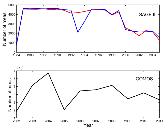
Fig. 1. The number of SAGE II sunrise (red) /sunset (blue) measurements for 1984–2005 and GOMOS nighttime measurements (black) for 2002–2011.
