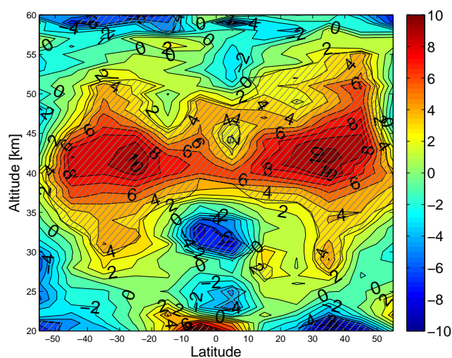
Fig. 16. The change in ozone trends in % per decade between the periods 1997–2011 and 1984–1997 at different latitudes. Shaded areas show regions where trend differences are statistically different from zero at the 95 % level.
