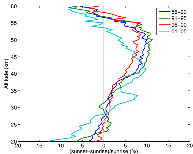
Fig. 4. The SAGE II ozone median of sunrise measurements compared to the median of sunset measurements for 5 yr periods in the tropics (10° S–10° N).
