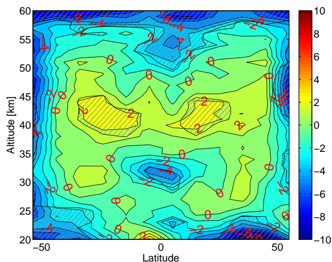
Fig. 15. The ozone trend in % per decade for different latitudes for 1997–2011. Shaded areas show regions where trends are statistically different from zero at the 95 % level.
