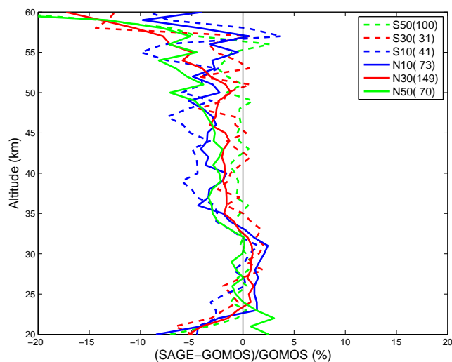
Fig. 7. The percent differences between SAGE II sunrise and GOMOS nighttime measurements in 20° latitude bands. The line labels show the centers of the latitude bands and the number of collocations.
