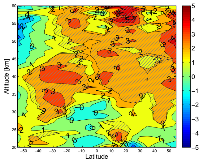
Fig. 13. The relative contribution of the solar proxy (%) with respect to the constant term for 1984–2011. Shaded areas show regions where trends are statistically different from zero at the 95 % level.
