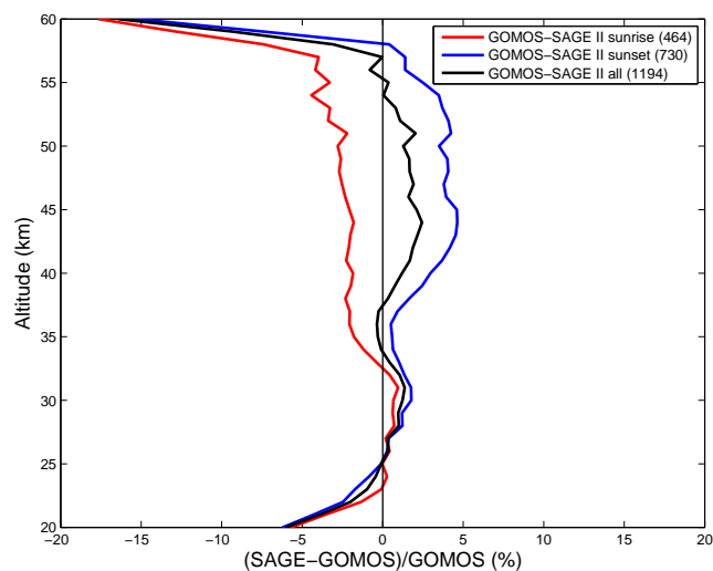
Fig. 3. The percent difference between SAGE II and GOMOS measurements for the collocations in 2002–2005. The corresponding differences between SAGE II sunrise and sunset measurements are also shown. The line labels show the number of collocations.
