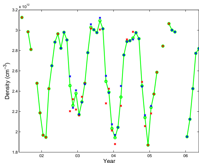
Fig. 10. An example of the combined SAGE II and GOMOS data sets at 30 km between 40–50° N. Red crosses indicate SAGE II data, blues crosses indicate GOMOS data, and the green line with circles indicates the combined data (gaps in the line are due to missing data).
