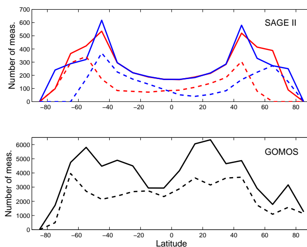
Fig. 2. Latitude distributions of SAGE II (top) and GOMOS (bottom) measurements. Notation: Solid and dashed red: SAGE II sunrise for 1985 and 2004, solid and dashed blue: SAGE II sunset for 1985 and 2004, solid and dashed black: GOMOS for 2004 and 2010.
