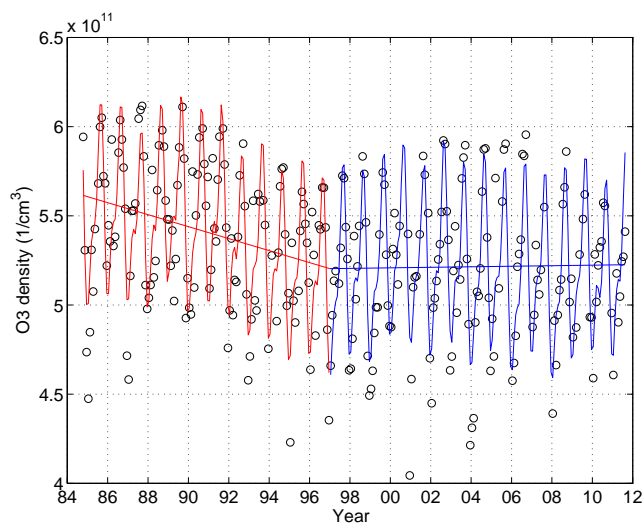
Fig. 12. An example of the fit at 40 km between 40–50° N for the combined SAGE II–GOMOS monthly data. The data points are black circles. The inflection year is 1997. The red solid curve and red line represent the fit and linear trend for 1984–1997, respectively. The blue solid curve and blue line represent the fit and linear trend for 1997–2011, respectively.
