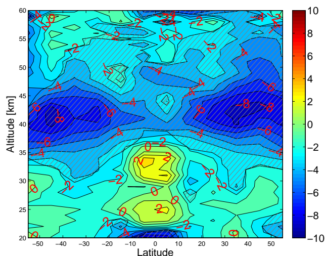
Fig. 14. The ozone trend in % per decade for different latitudes for 1984–1997. Shaded areas show regions where trends are statistically different from zero at the 95 % level.
