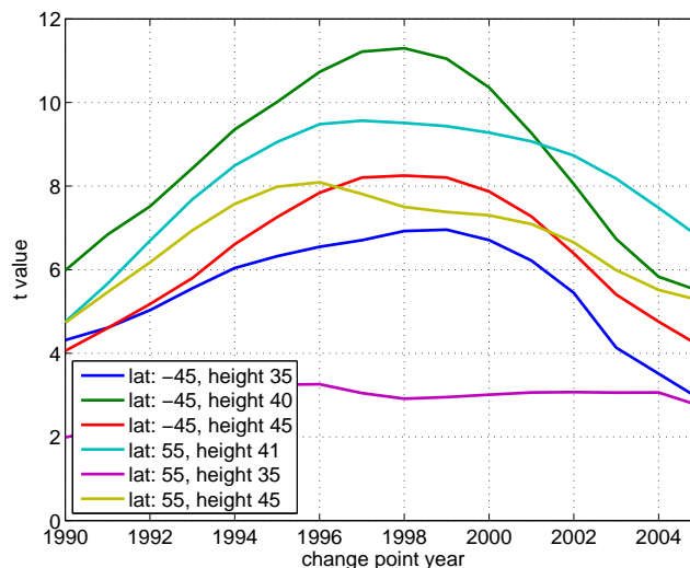
Fig. 11. The t values for the difference of trend terms at different latitudes and altitudes as a function of the inflection year.
