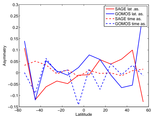
Fig. 6. The mean latitudinal and temporal asymmetries as a function of latitude.
