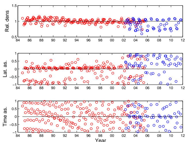
Fig. 5. Asymmetries of the monthly time series in the 50–60° N latitude range. Top: GOMOS and SAGE II ozone densities at 40 km scaled by the median of the combined time series at 40 km, middle: latitude asymmetries, bottom: time asymmetries. Red circles are for SAGE II and blue circles for GOMOS data.
