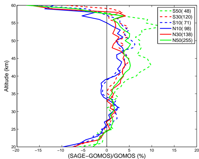
Fig. 8. The percent differences of SAGE II sunset and GOMOS nighttime measurements in 20° latitude bands. The line labels show the centers of the latitude bands and the number of collocations.
