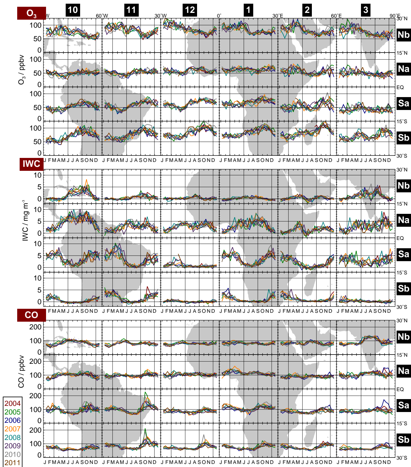
Fig. 1. MLS 215 hPa O_3 (upper), cloud ice (middle, indicative of convection), and CO (lower) observations from 90^\circ\text{W} to 90^\circ\text{E} . Each cell shows timeseries of biweekly averages of MLS measurements in the geographic region covered by the cell. Line colors denote year, as shown in the legend at the bottom left. Numbers and letters in black boxes along the top and right edges identify regions for discussion in the text (e.g., 3Nb is the box encompassing much of India).
