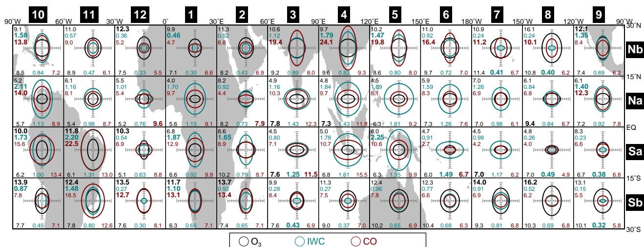
Fig. 8. Map summarizing the S (height of each ellipse) and V (width of each ellipse) statistics for \text{O}_3 (black), IWC (cyan) and CO (red). The ‘crosshairs’ give the scale, with major ticks at 10 and 20 ppbv for \text{O}_3 and CO and 1 and 2 \text{mg m}^{-3} for IWC. Corresponding (color coded) values of S are shown in the top left of each panel (large/bold type indicates ‘distinctly seasonal’ cases where S > 1.5V ), with V shown along the bottom edge (where large/bold type indicates ‘mostly interannual’ cases having V > 1.5S ).
