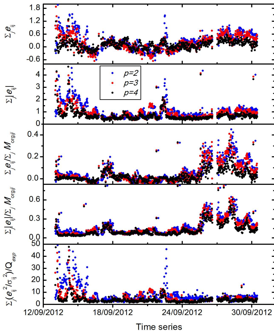
Fig. S4. Time series of the model residuals e_{ij} for the PMF analysis with FPEAK = zero.
