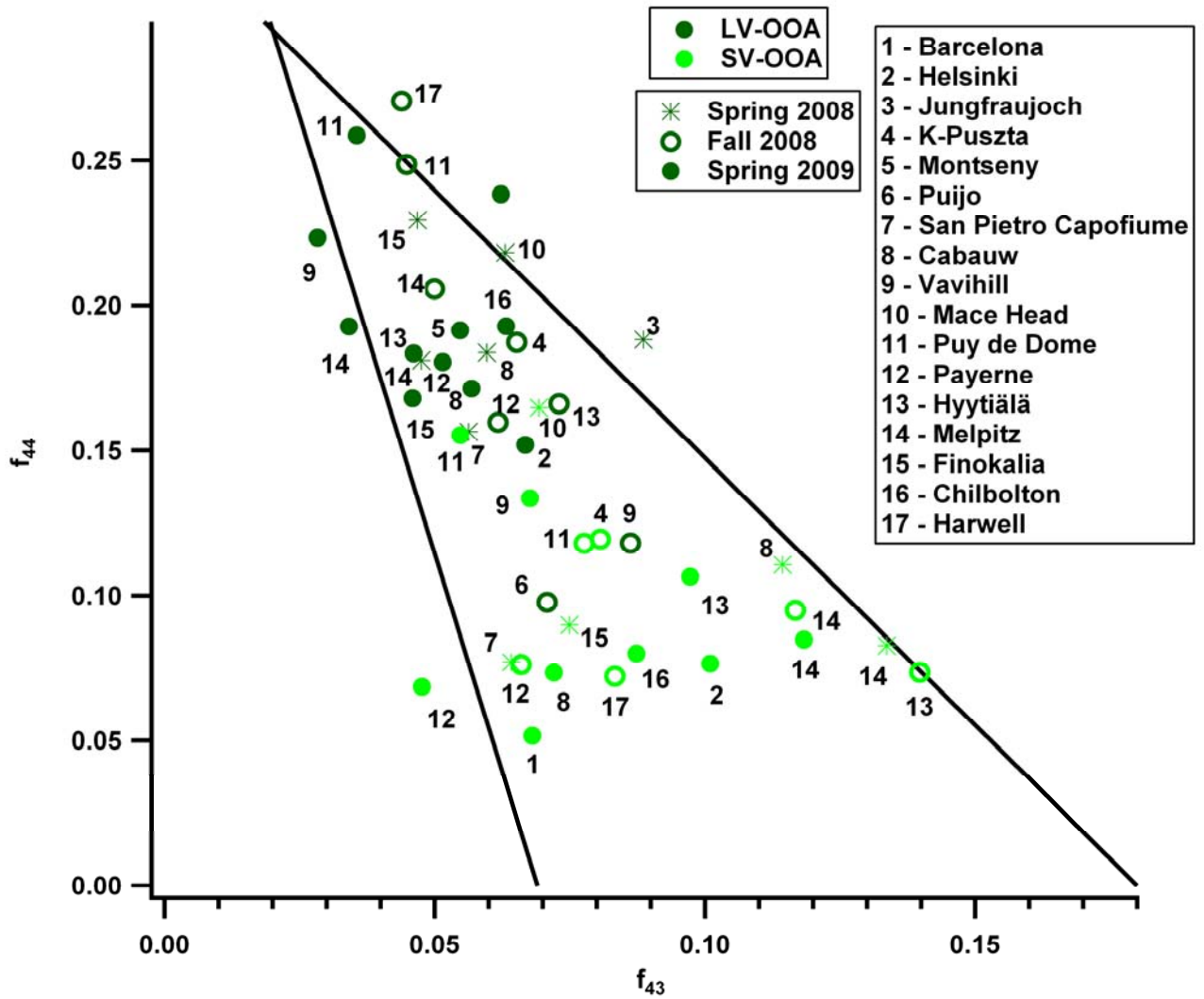
Fig. SI-4: f_{44} vs. f_{43} triangle plot.
