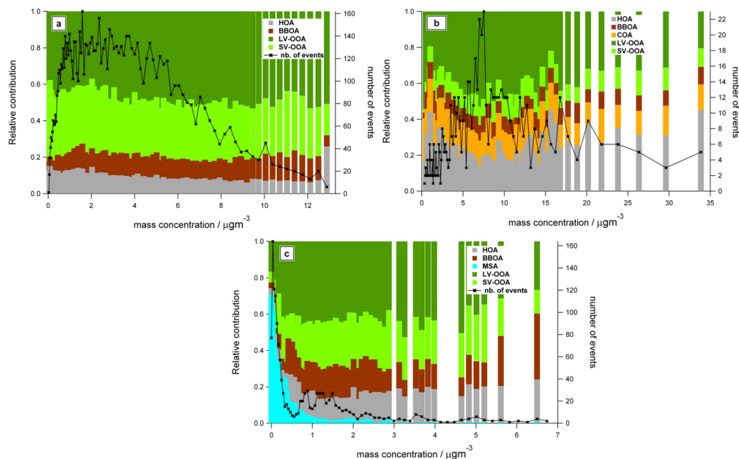
Figure 5. Relative organic source contributions as a function of total organic concentrations. Average plot over all the seasons and rural sites (a), Barcelona only (b), and average plot for marine sites (c).
