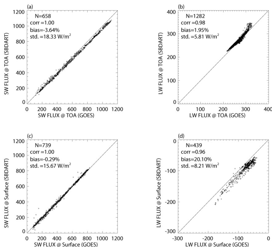
Figure 3. Santa Barbara DISORT Atmospheric Radiative Transfer (SBDART)-modeled flux as a function of satellite-retrieved flux for (a) SW fluxes at the TOA, (b) LW fluxes at the TOA, (c) SW fluxes at the surface, and (d) LW fluxes at the surface. Units are \text{W m}^{-2} . Standard deviation, bias, correlation coefficient, and number of data points ( N ) are given.
