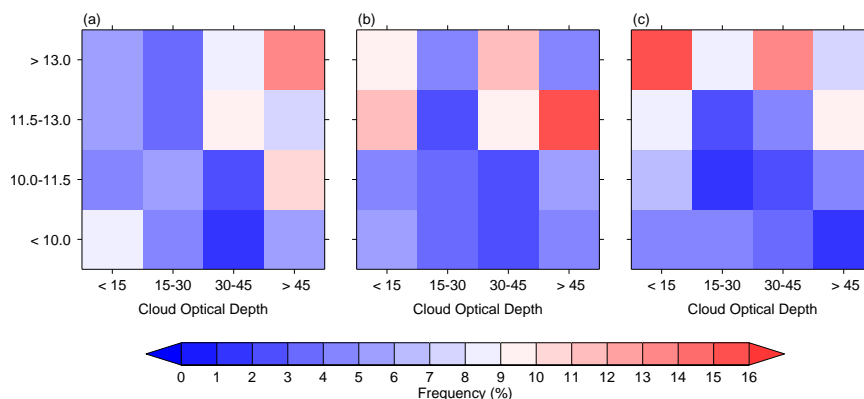
Figure 6. Cloud frequency of occurrence at three levels of CN concentration: (a) 0–2000 \text{cm}^{-3} , (b) 2000–4000 \text{cm}^{-3} , and (c) 4000–6000 \text{cm}^{-3} . Data are binned according to COD and cloud-top height.
