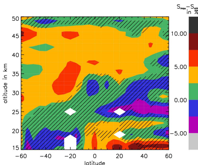
Fig. A2. Latitude–altitude plot of solar cycle signal in SCIAMACHY limb O 3 : latitude range from 60° N to 60° S, altitude range from 15 to 50 km. Significances at the 2 \sigma level are non-hatched areas. The solar cycle signal is expressed as the solar max minus min change of O 3 (more detailed explanation in the text). It is scaled in relative units with respect to the mean value of the underlying time series. The period of August 2002–April 2012 is considered. Legend on the right: solar max minus min change in units of %.
