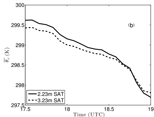
Figure 3. Observed temporal evolution of the virtual potential temperature at 2.23 m (solid line) and 3.23 m (dashed line) during the evening transitions on (a) 30 June and (b) 1 July 2011.
