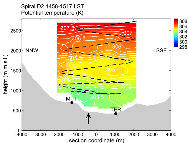
Figure 10. As in Fig. 7 but for spiral D2. The horizontal coordinate marks the local cross-valley direction for the Lakes Valley. The cross section is taken about 2 km upstream of the Terlago saddle ridge, whose lowest point's projection is indicated by the black arrow. The projection of MTT's and TER's position is also indicated (black dots).
