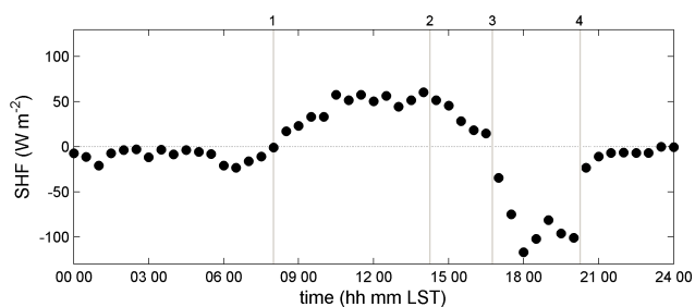
Figure 11. Vertical sensible heat flux (SHF) for 23 August 2001, from eddy covariance analysis of ultrasonic anemometer measurements (averaging interval: 30 min) collected at RON2. The vertical grey lines indicate (1) beginning of the morning heating, (2) beginning of the SHF decrease at the arrival of the Ora del Garda, (3) shift to negative SHF and (4) end of the phase characterized by large negative SHF.
