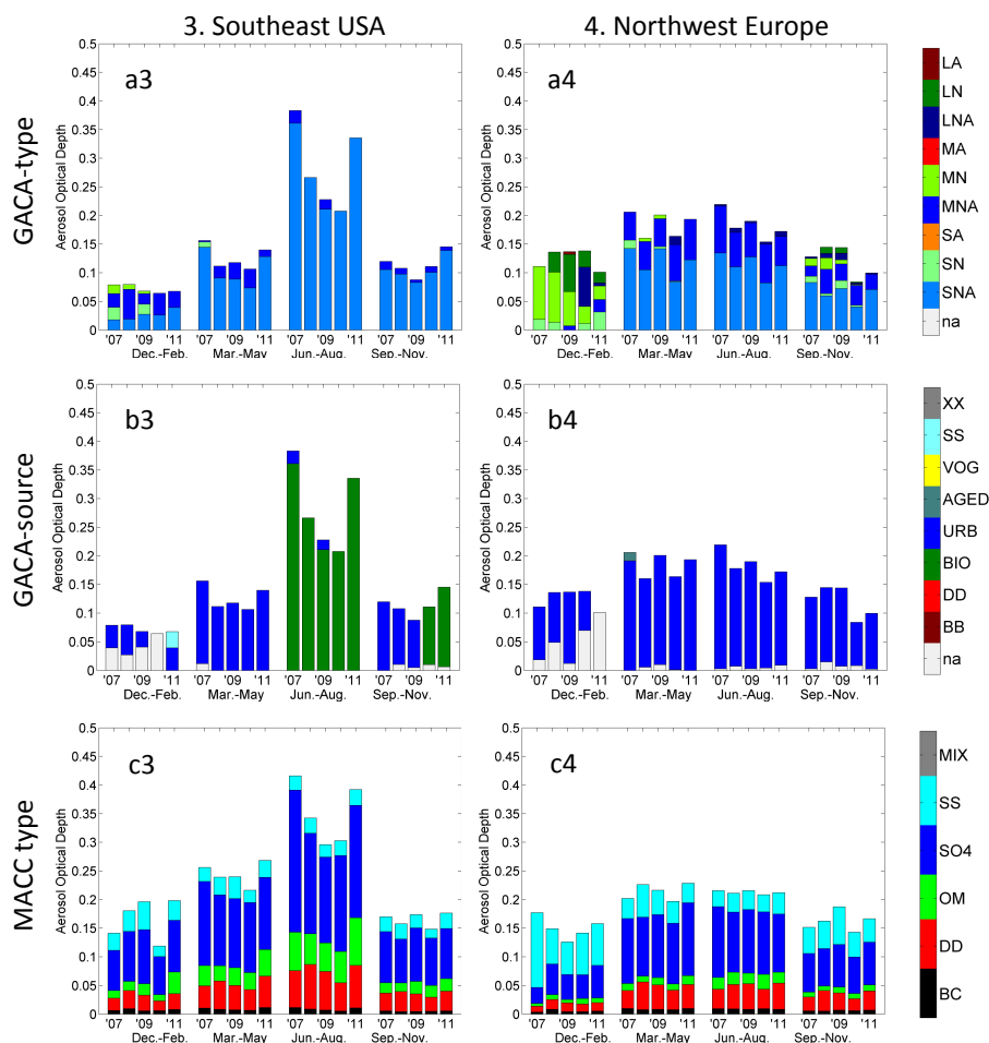
Figure 11. Seasonal cycles of global aerosol type and source according to GACA and MACC for 5^{\circ} \times 5^{\circ} regions in southeastern USA ( 30\text{--}35^{\circ} N, 80\text{--}85^{\circ} W) and northwestern Europe ( 48\text{--}53^{\circ} N, 3\text{--}8^{\circ} E). See Fig. 10 for details.
