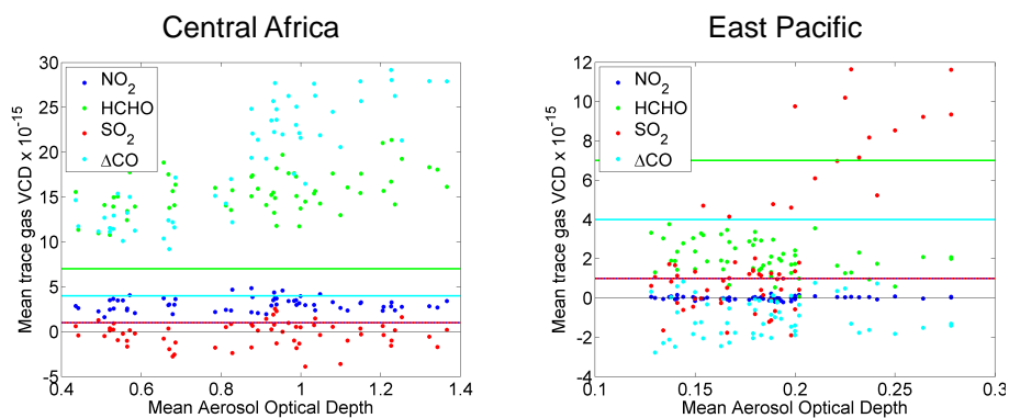
Figure 3. Relationship between 1^\circ \times 1^\circ monthly mean values of AOD and trace gas columns (in molec \text{cm}^{-2} ) for a region in central Africa ( 2\text{--}4^\circ S, 18\text{--}20^\circ E; left panel) and in the eastern Pacific Ocean ( 16\text{--}18^\circ N, 162\text{--}164^\circ W; right panel) for July–August 2007–2011. Dots depict \text{NO}_2 (blue), HCHO (green), and \text{SO}_2 (red) VCDs and excess CO VCDs (light blue, scaled by a factor of 0.01) and their respective thresholds. The threshold values of \text{NO}_2 and \text{SO}_2 are identical (dotted blue and red lines). Note the differences in y axis scales.
