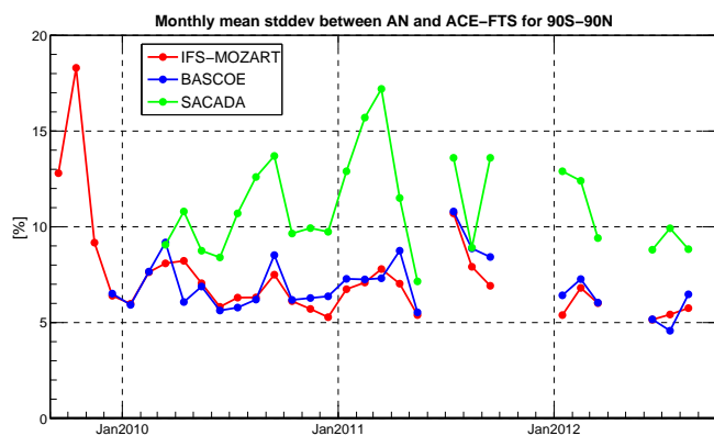
Figure 5. Comparison of the global (i.e. from 90^{\circ} S to 90^{\circ} N) monthly mean standard deviation between IFS-MOZART (red), BASCOE (blue), and SACADA (green) with ACE-FTS (analysis minus observations) in %, for the [200,5]hPa pressure bin, for the period September 2009 to September 2012. Standard deviations for levels with less than 20 observations are omitted. Note that standard deviations are not weighted by the cosine of the latitude.
