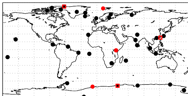
Figure 1. Location of all stations used in this paper. O 3 sondes are indicated as filled black circles. The ones selected for a more detailed discussion have been marked in red: Ny-Ålesund (79° N, 12° E) in the Arctic, Nairobi (1.27° S, 36.8° E) in the tropics, and Neumayer (70.65° S, 8.25° W) in the Antarctic. The three sites selected for the total ozone column (TOC) discussion are indicated by the red squares.
