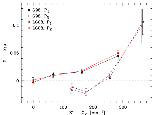
Figure 4. Over- and underpopulation of the upper rotational levels of the P -branch OH lines relative to a regression line based on the first three P_1 and P_2 lines. The abscissa shows the energy difference in \text{cm}^{-1} of an upper rotational level E' to the lowest level G_v . The ordinate exhibits the natural logarithm of a population ratio. The data points show the mean values and mean errors of the four investigated P_1 (filled symbols and solid lines) and P_2 lines (open symbols and dashed lines) for the OH bands (4-1), (5-2), (6-2), and (7-4). The results for the G98 and LG08 line parameters are marked by circles and diamonds, respectively.
