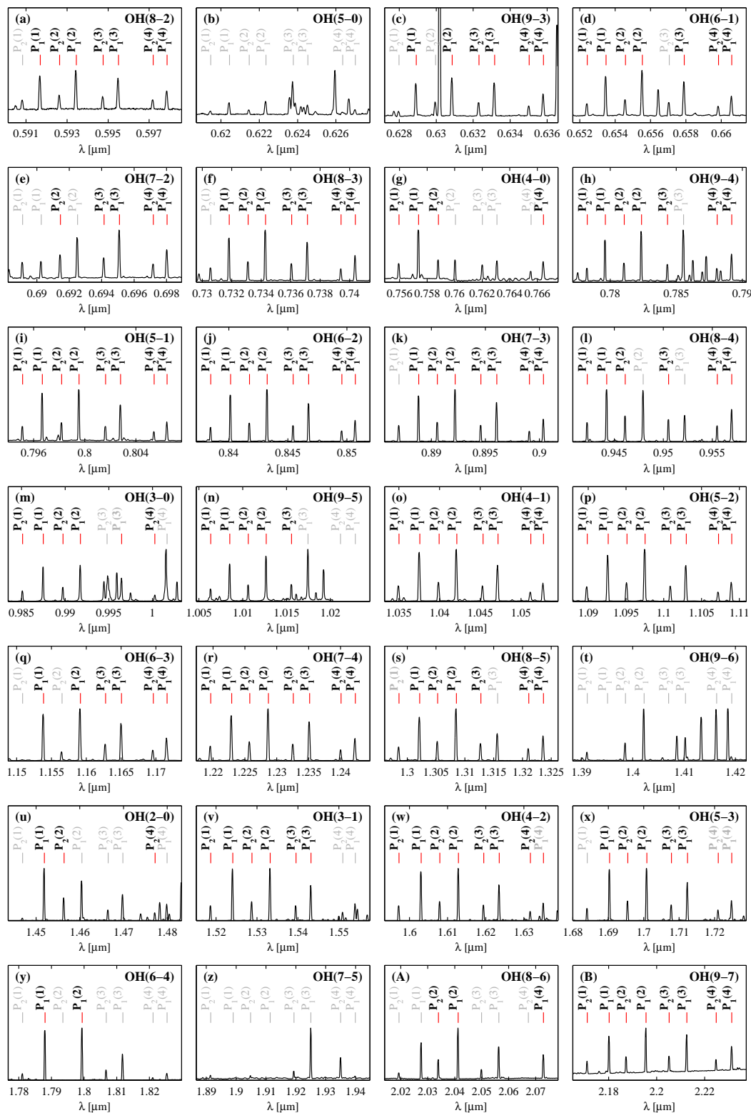
Figure 2. P -branch lines of the OH bands used in this study. The displayed spectrum is the pixel-related median of the 240 X-shooter VIS- and NIR-arm observations which cover all bands and where a reliable flux calibration could be performed in the K band. Lines with black labels were used for the derivation of temperatures. Lines with grey labels were excluded from this study. An exception are those with red marker lines. They were considered for the T_{\text{rot}} correction due to differences in the sets of lines available for each band.
