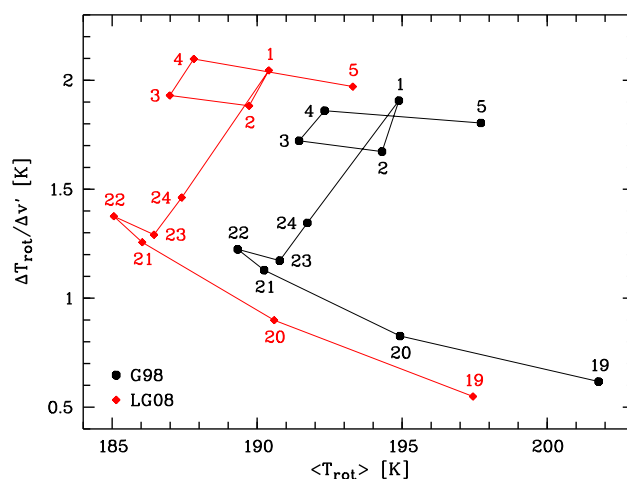
Figure 10. Change of T_{\text{rot}} with v' \Delta T_{\text{rot}}/\Delta v' (slope of regression line) as a function of the average \langle T_{\text{rot}} \rangle of all v' for local time bins centred on the hour (see labels). The plot is based on the T_{\text{rot}}(v') of the individual spectra. Results are shown for the G98 (black filled circles) and LG08 line parameters (red filled diamonds), respectively.
