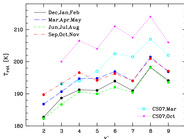
Figure 12. Rotational temperature T_{\text{rot}}(v') as a function of v' for different meteorological seasons. The plot details are similar to those of Fig. 9. In addition, we show the Mauna Kea (19.8° N) mean T_{\text{rot}}(v') for March and October 2000 by Cosby and Slanger (2007).
