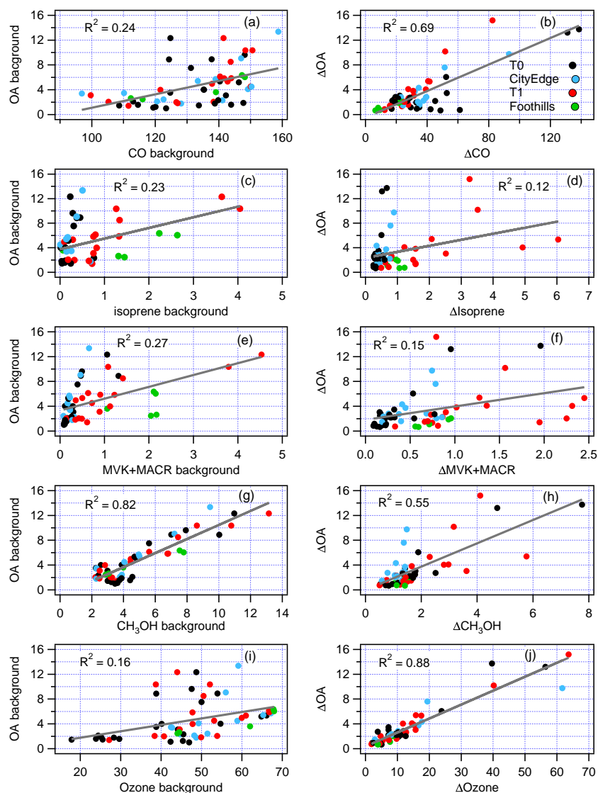
Figure 7. OA as a function of CO, isoprene, MVK + MACR, CH 3 OH, and O 3 for 56 transects. Background concentrations in panels on left-hand side; \Delta Concentrations on the right-hand side. Color legend in panel (b) identifies data according to location. Gray lines are linear least-squares fits with R^2 given in each panel.
