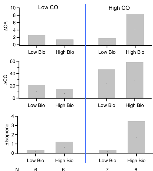
Figure 8. Values of \Delta\text{OA} , \Delta\text{CO} , and \Delta\text{Isoprene} for 4 subsets of transects. Pairs of bars labeled low CO and high CO have \Delta\text{CO} values that are below the 33rd percentile and above the 67th percentile, respectively. Bars labeled low Bio and high Bio have \Delta\text{Isoprene} values that are below the 33rd percentile and above the 67th percentile, respectively. Number of transects in each subset given at bottom. \Delta\text{CO} ratio and \Delta\text{Bio} ratio give effects of precursor mixing ratio on an A–B interaction relative to the expectation that \Delta\text{OA} is a bilinear function of \Delta\text{CO} , and \Delta\text{Bio} : \Delta\text{CO} ratio is (\Delta\text{CO}: \text{high CO, high Bio}) / (\Delta\text{CO}: \text{high CO, low Bio}) . \Delta\text{Bio} ratio is (\Delta\text{Bio}: \text{high CO, high Bio}) / (\Delta\text{Bio}: \text{high CO, low Bio}) .
