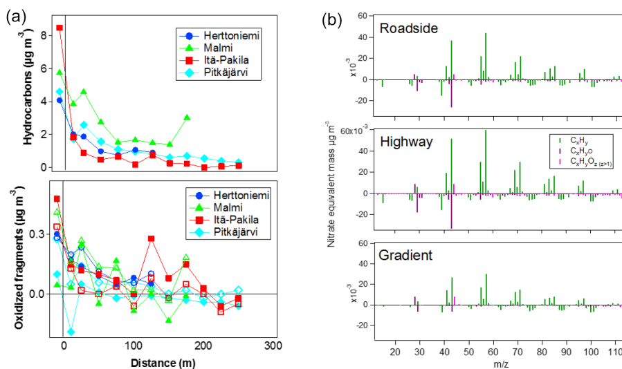
Figure 6. Concentrations of hydrocarbon fragments ( C_xH_y^+ ) and oxidized organic fragments ( C_xH_yO^+ and C_xH_yO_z^+ , Z_{>1} ) measured at the four sites (a), and the average mass spectra for highway, roadside, and gradient at Pitkajärvi (b). Solid markers refer to organic fragments with one oxygen atom and open markers to organic fragments with more than one oxygen atoms in lower figure of (a). In (a) zero distance refers to the roadside and negative value driving on the highway. Background values were subtracted both from the measured concentrations and mass spectra.
