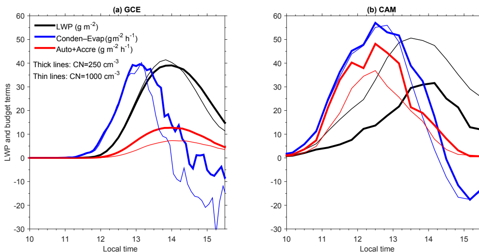
Figure 3. LWP and the column-integrated LWP source and sink terms from the cases with surface aerosol number concentration equal to 250\text{ cm}^{-3} (thick lines) and 1000\text{ cm}^{-3} (thin lines) for (a) GCE and (b) CAM.
