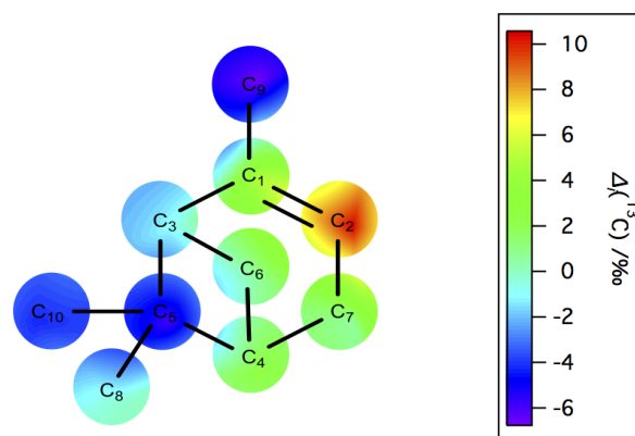
Figure 7. Heat map of \Delta_i(^{13}\text{C}) in \alpha -pinene (Sigma-Aldrich, lot MKBQ6213V) relative to its bulk isotopic composition; see Table 1. The boundary of the image was set to \Delta_i(^{13}\text{C}) = 0 , i.e. the bulk isotopic composition. A large enrichment is visible at the double bond (C 2 ), and large depletions are visible at positions C 5 and C 9 where isotopic substitution is expected to reduce the molar volume significantly. C atoms are numbered in order of decreasing ^{13}\text{C} chemical shifts in the ^{13}\text{C} NMR spectrum.
