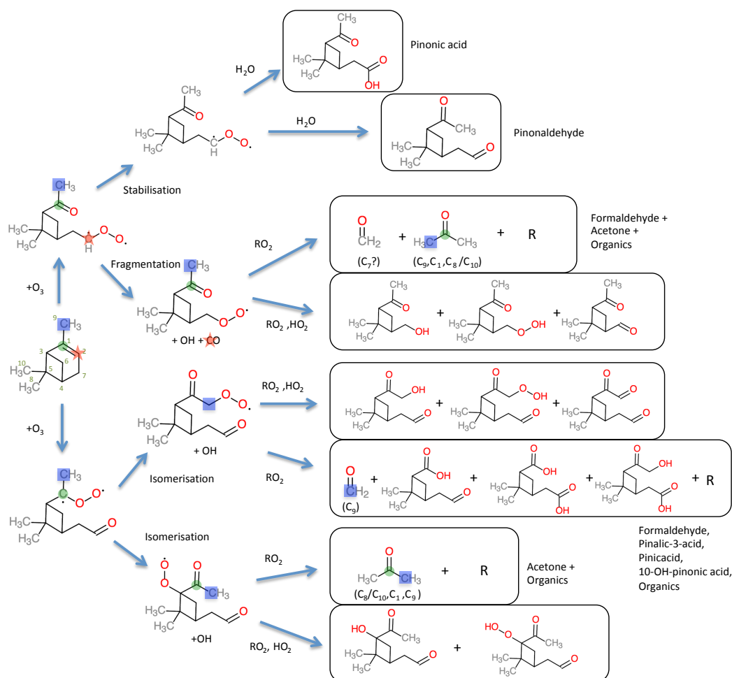
Figure 1. Reaction scheme of \alpha -pinene ozonolysis, based on (Camredon et al., 2010), using the reaction mechanism of MCMv3.1. The boxes show first-generation products, while subsequent dimer formation and oligomerisation are not shown. The O : C ratio typically increases as oxidation proceeds (i.e. oxygen addition via functionalisation). Large, oxygenated product compounds (e.g. pinonic acid, pinonaldehyde) have lower vapour pressures and partition to the particle phase. Small, volatile products including HCHO, acetone, and CO result from fragmentation processes and partition to the gas phase. The coloured symbols highlight how the parent \alpha -pinene's atoms (denoted in brackets) can form small reaction products including CO, HCHO, and acetone. The symbol colours were chosen based on the heat map in Fig. 7.
