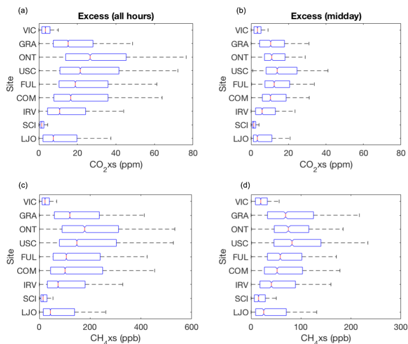
Figure 6. Boxplot of enhancements (CO 2 xs and CH 4 xs) in the LA megacity observed during 2015 relative to the San Clemente Island background estimate. Results are shown for CO 2 xs (a, b) and CH 4 xs (c, d) and for all hours (a, c) and mid-afternoon hours (12:00–16:00 LT, b, d). The sites are arranged by latitude from north to south (top to bottom): Victorville (VIC), Granada Hills (GRA), Ontario (ONT), downtown LA (USC), California State University, Fullerton (FUL), Compton (COM), University of California, Irvine (IRV), San Clemente Island (SCI), and La Jolla (LJO). Boxes outline the 25th and 75th percentiles of the sample data, respectively, and red horizontal lines show the median values at each site. Values outside the 25th and 75th percentiles are not shown here but are plotted in Fig. S11. (Note: only positive enhancements are shown. Results for the ONT site are for September to December 2015, while all other results are annual averages. Results from the USC site are shown for the G2401 analyzer only).
