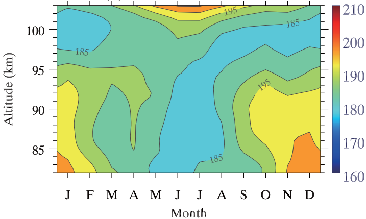
(b) SABER temperature
