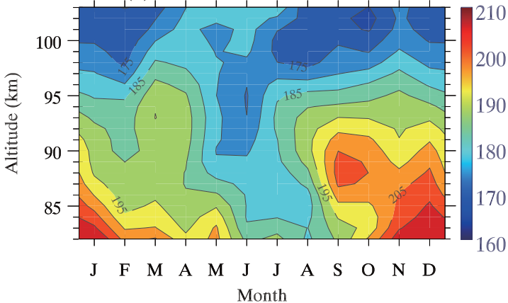
(a) USTC lidar temperature
