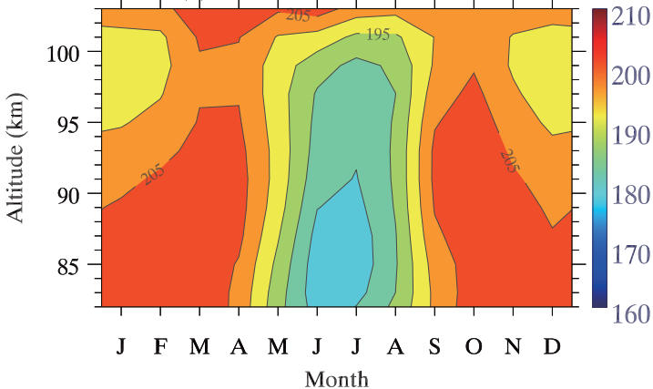
(c) WACCM temperature
