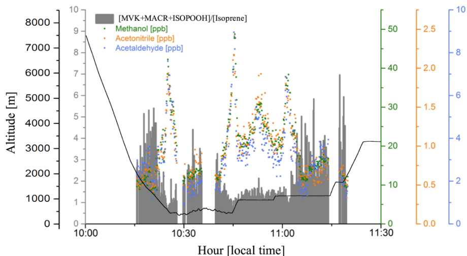
Figure 7. Methanol (green dots), acetonitrile (orange dots), and acetaldehyde (blue dots) mixing ratios (ppbv), and the [\text{MVK} + \text{MACR} + \text{ISOPOOH}] / [\text{isoprene}] ratio (gray bars), during a plume interception along the flight track B732 in different altitudes.
