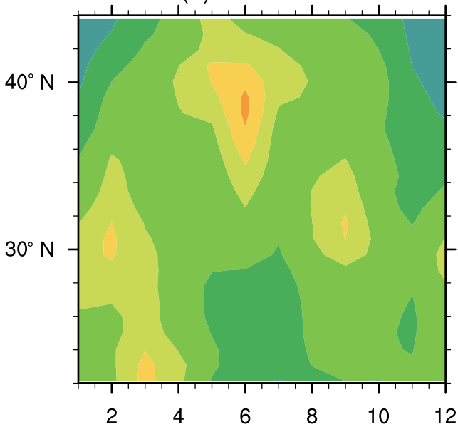
(c) MODIS AOD
