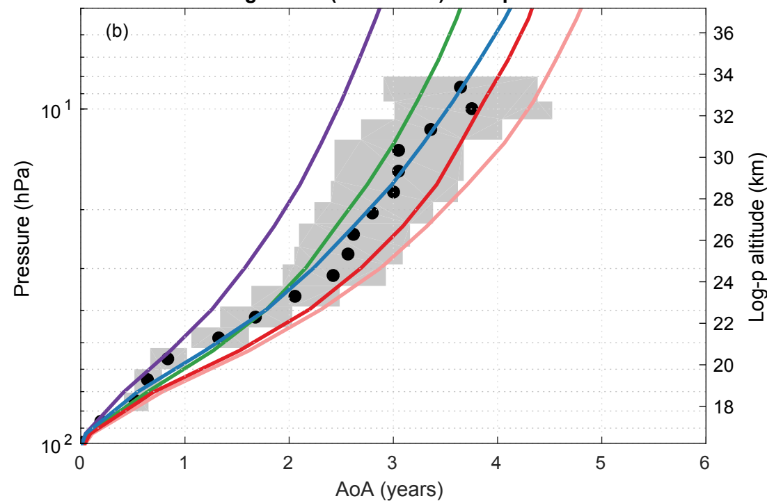
Mean age of air (2002–2007) in tropics
