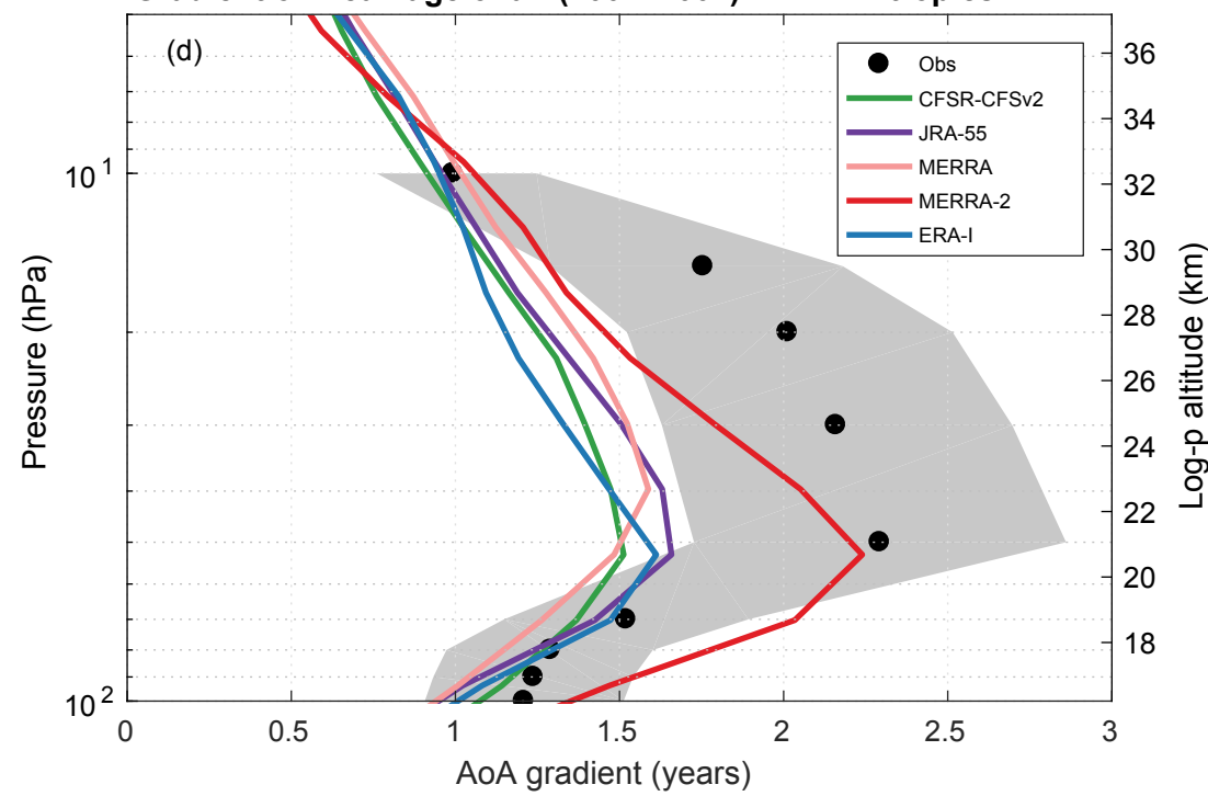
Gradient of mean age of air (2002–2007): MLNH – tropics
