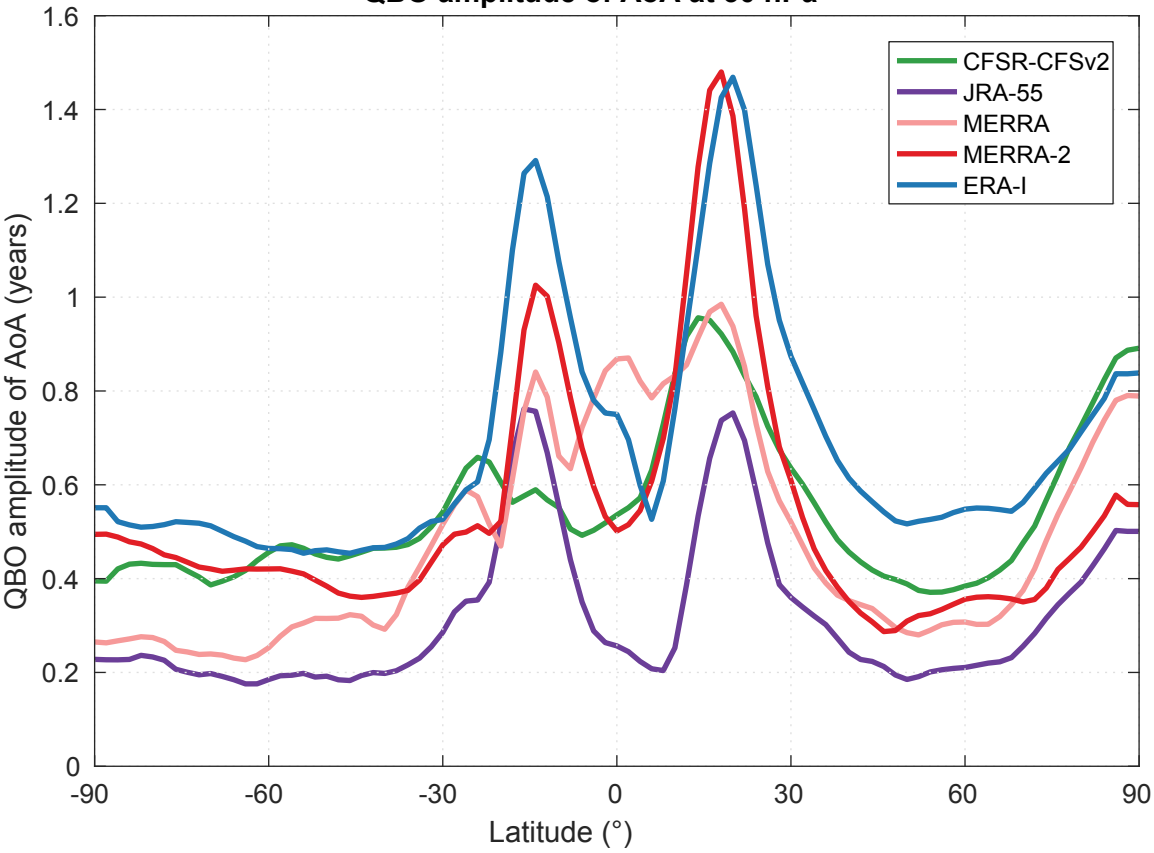
QBO amplitude of AoA at 30 hPa
