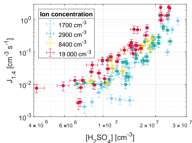
Figure 5. Nucleation rates as a function of sulfuric acid concentration and ion concentration. The error bars represent 1\sigma standard deviation on the [\text{H}_2\text{SO}_4] and the 95 % confidence interval on the nucleation rate.
