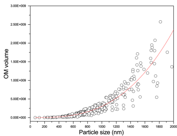
Figure S6 OM volume vs particle size in the analyzed particles. Unite of OM volume is nm 3
