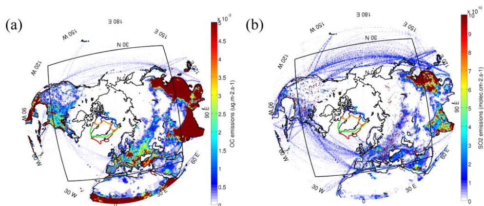
Figure S2 OC (a) and \text{SO}_2 (b) Emission intensity in Arctic area and 24h back trajectories on August 11, 12, 14, and 15, 2012.
