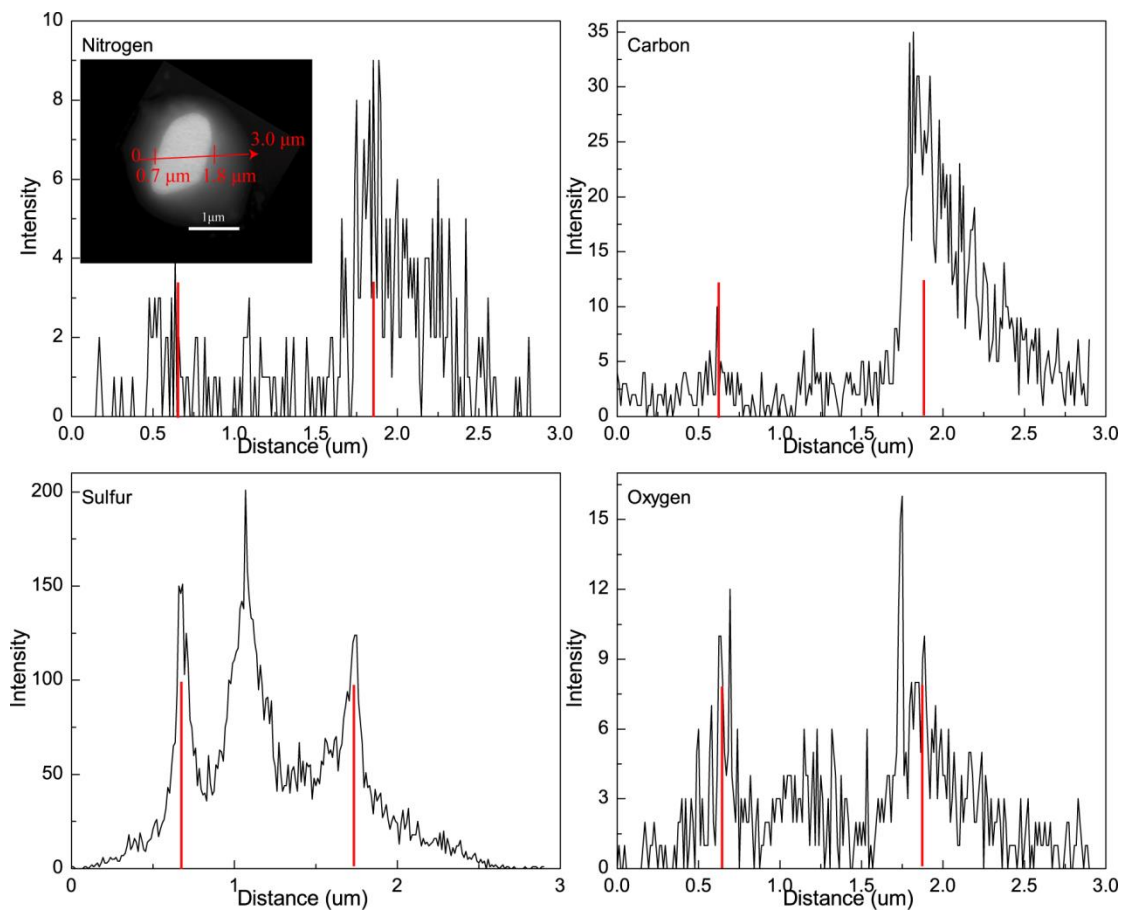
Figure S4 Elemental profile of individual particle containing sulfate with organic coating.
