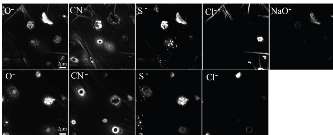
Figure S1 NanoSIMS based on intensity threshold maps of single ion in arctic aerosol particles in different samples. The mixture of OM and sulfate were identified based on \text{CN}^- and \text{S}^- . The aged sea salt particles containing \text{CN}^- and \text{S}^- were excluded based on \text{Cl}^- and \text{NaO}^- .
