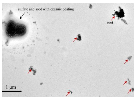
Figure S5 Low magnification TEM images of sulfate and soot particles
