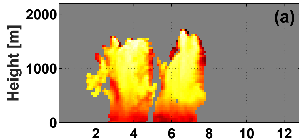
BOMEX-250: RH [%] cross-section
