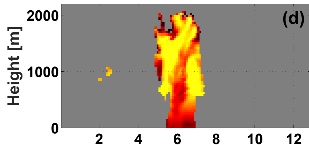
BOMEX-2000: RH [%] cross-section
