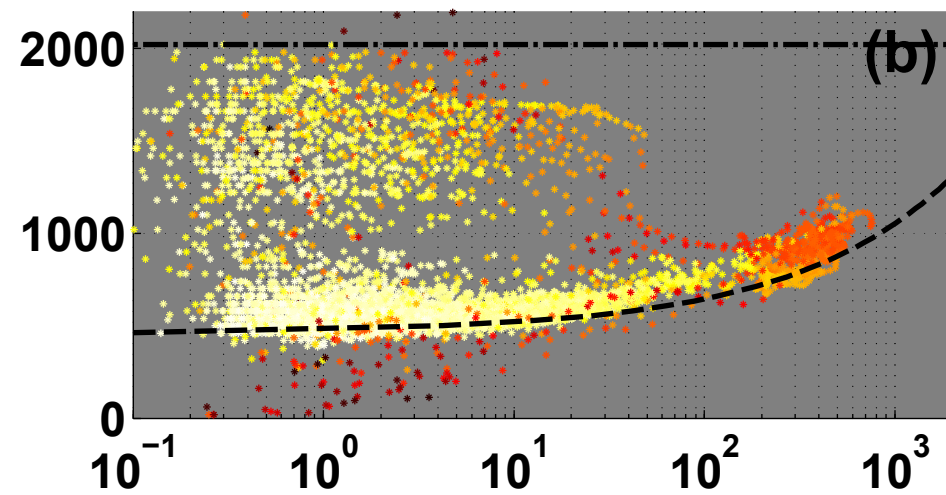
BOMEX-250: margin mean RH [%]
