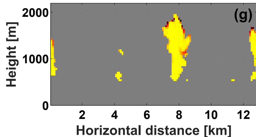
BOMEX-2000: RH [%] cross-section
