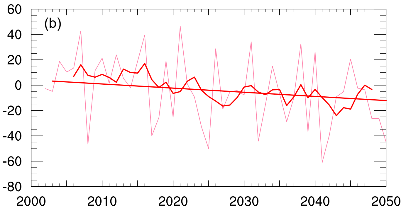
\Delta PCO (SEN-REF), LS, Antarctic, September
