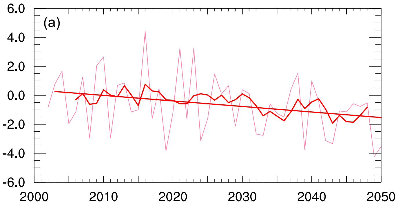
\Delta PCO (SEN-REF), US, Antarctic, September
