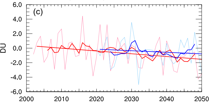
\Delta PCO (SEN-REF), US, Antarctic, September
