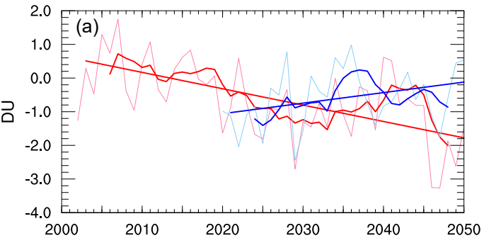
\Delta TCO (SEN-REF), annual near-global mean
