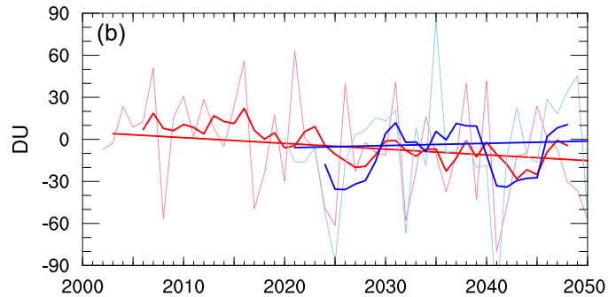
\Delta TCO (SEN-REF), Antarctic, September
