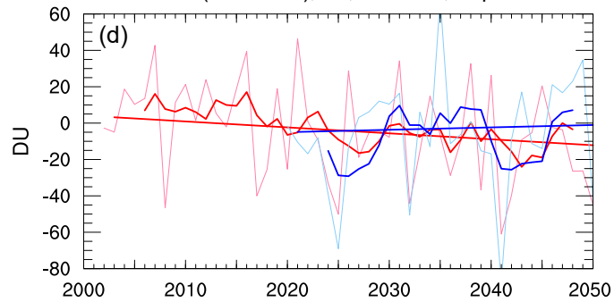
\Delta PCO (SEN-REF), LS, Antarctic, September
