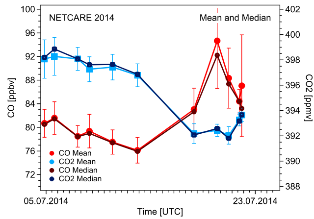
Figure S 6. CO (red) and CO 2 (blue) data for NETCARE 2014. Shown are the respective mean and median value of all data points on the individual flight.
