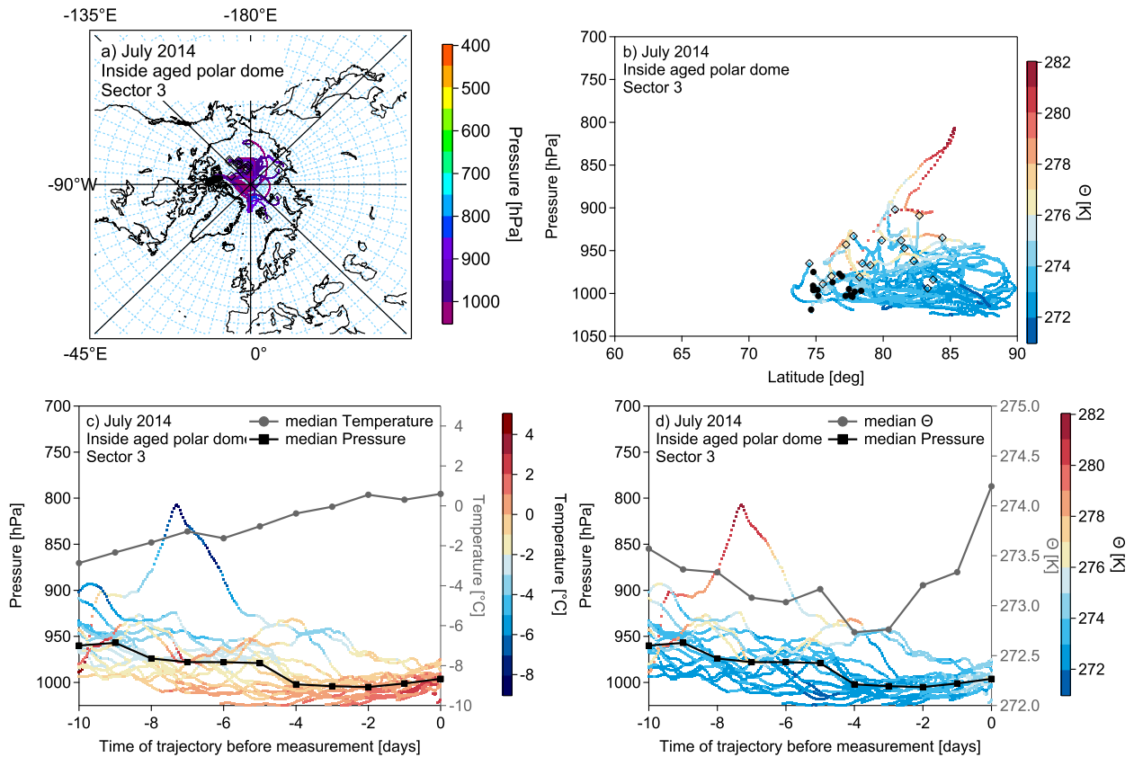
Figure S3. (a) Trajectories of the most dominant sector 3 for air masses inside the aged polar dome. The color code represents the pressure along the trajectories. (b) The same trajectories as in (a) as a function of pressure and latitude, color coded by potential temperature. In both (a) and (b) black circles denote the initialization point of the trajectory along the flight track. The black open squares show the position of the trajectory 10 days back in time. Panels (c) and (d) show height-time cross-sections with pressure representing the altitude of the trajectories (left axis) for the trajectory evolution over the 10 days of travel with the color code denoting the temperature (c) and potential temperature (d). The black line marks the median pressure of the trajectory cluster at the individual time steps and the grey line indicates the median temperature and median potential temperature, respectively. Note that only every 20th trajectory is plotted for figure clarity.
