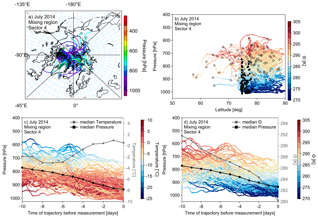
Figure S 4. (a) Trajectories of the most dominant sector 4 for air masses inside the mixing region. The color code represents the pressure along the trajectories. (b) The same trajectories as in (a) as a function of pressure and latitude, color coded by potential temperature. In both (a) and (b) black circles denote the initialization point of the trajectory along the flight track. The black open squares show the position of the trajectory 10 days back in time. Panels (c) and (d) show height-time cross-sections with pressure representing the altitude of the trajectories (left axis) for the trajectory evolution over the 10 days of travel with the color code denoting the temperature (c) and potential temperature (d). The black line marks the median pressure of the trajectory cluster at the individual time steps and the grey line indicates the median temperature and median potential temperature, respectively. Note that only every 20th trajectory is plotted for figure clarity.
