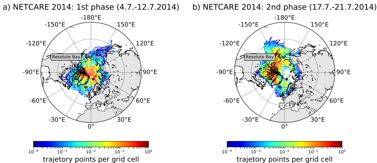
Figure S 1. Area weighted trajectory density during the different campaign phases in July 2014 (gridded by 1^{\circ} \times 1^{\circ} ). The colour code represents the amount of trajectory points per grid box weighted by the area of the grid box. The individual panels show the results for the first phase (a) and the second phase (b). The bold black dashed line denotes the Arctic circle.
