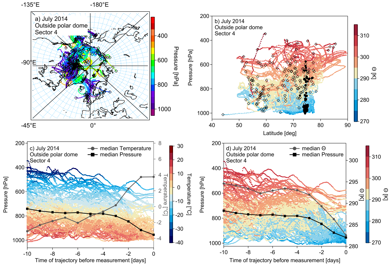
Figure S 5. (a) Trajectories of the most dominant sector 4 for air masses outside the polar dome. The color code represents the pressure along the trajectories. (b) The same trajectories as in (a) as a function of pressure and latitude, color coded by potential temperature. In both (a) and (b) black circles denote the initialization point of the trajectory along the flight track. The black open squares show the position of the trajectory 10 days back in time. Panels (c) and (d) show height-time cross-sections with pressure representing the altitude of the trajectories (left axis) for the trajectory evolution over the 10 days of travel with the color code denoting the temperature (c) and potential temperature (d). The black line marks the median pressure of the trajectory cluster at the individual time steps and the grey line indicates the median temperature and median potential temperature, respectively. Note that only every 20th trajectory is plotted for figure clarity.
