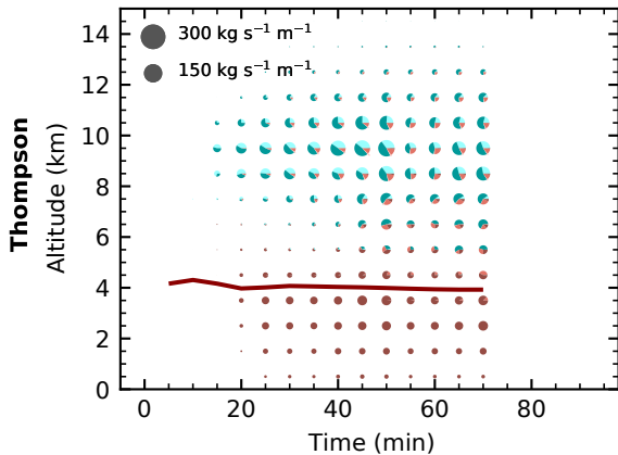
(c) THOM 50 cm -3
