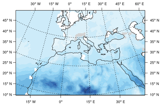
MISR
