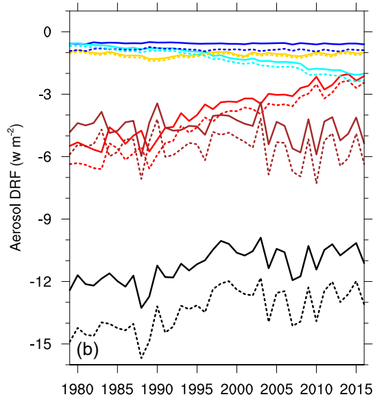
Mediterranean (TOA)
