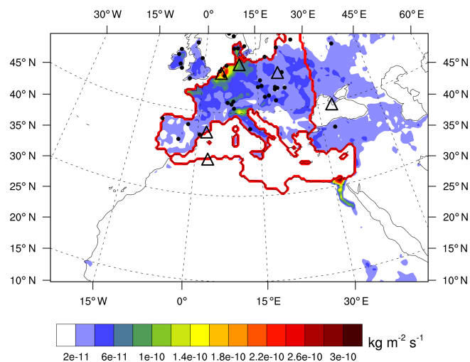
Figure 1. NH 3 emissions (CMIP6) over the period 1979–2016. The inner model domain represents 101 \times 153 points (without the bi-periodization and the relaxation zone). The different zones studied (Europe, Mediterranean) are represented in red. The observation data are symbolized by a black dot (EMEP stations) and by a black triangle (AERONET stations). The projection type used here is the Lambert conformal projection.
