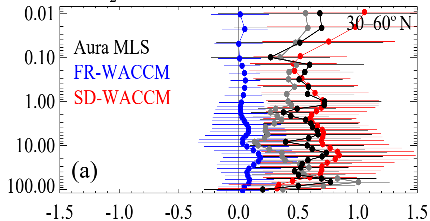
H 2 O trends for 2005–2014/2018
