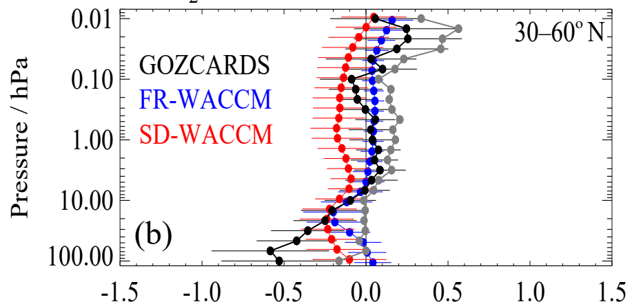
H 2 O trends for 1992–2010/2018
