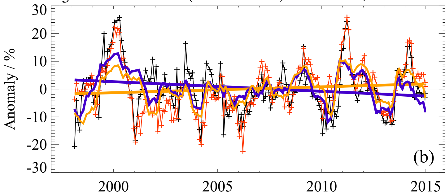
O 3 series and fits (1998–2014) at 68 hPa, 20° S–20° N
