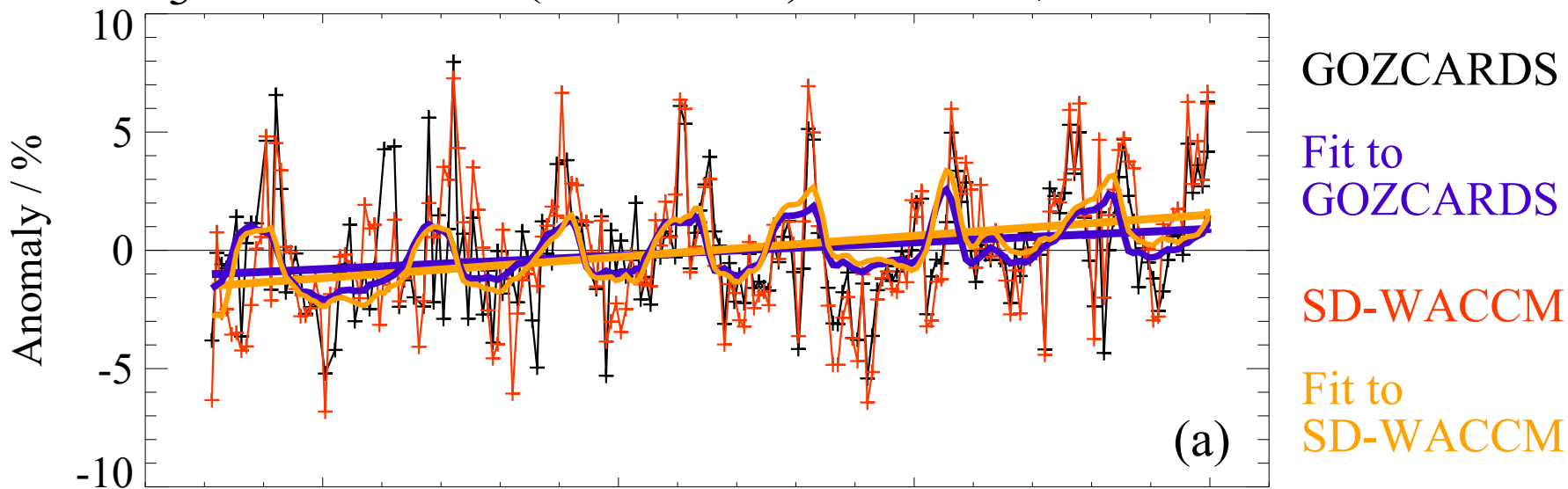
O 3 series and fits (1998–2014) at 68 hPa, 20° S–20° N
