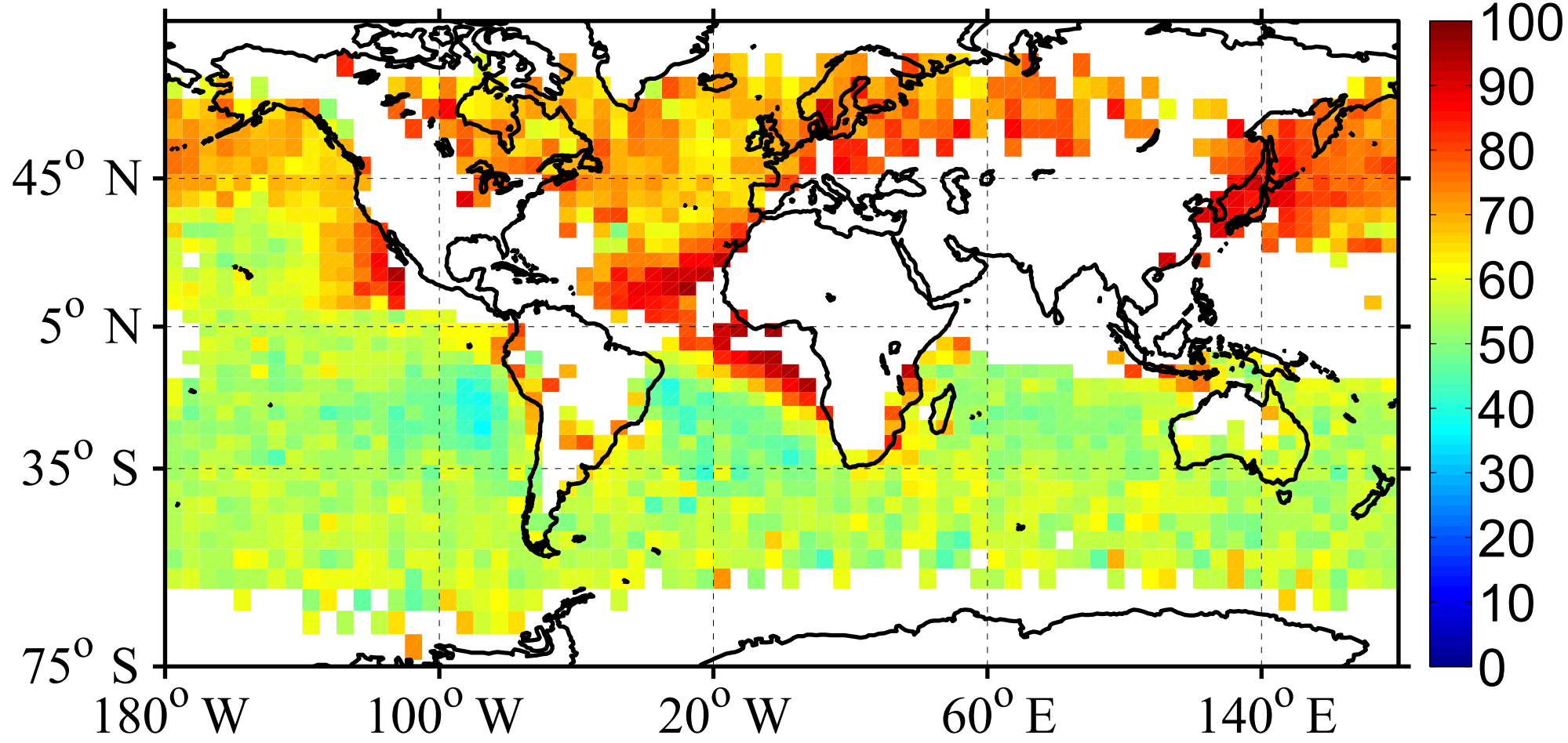
JJA max: 97 % median: 58 % mean: 58 %
