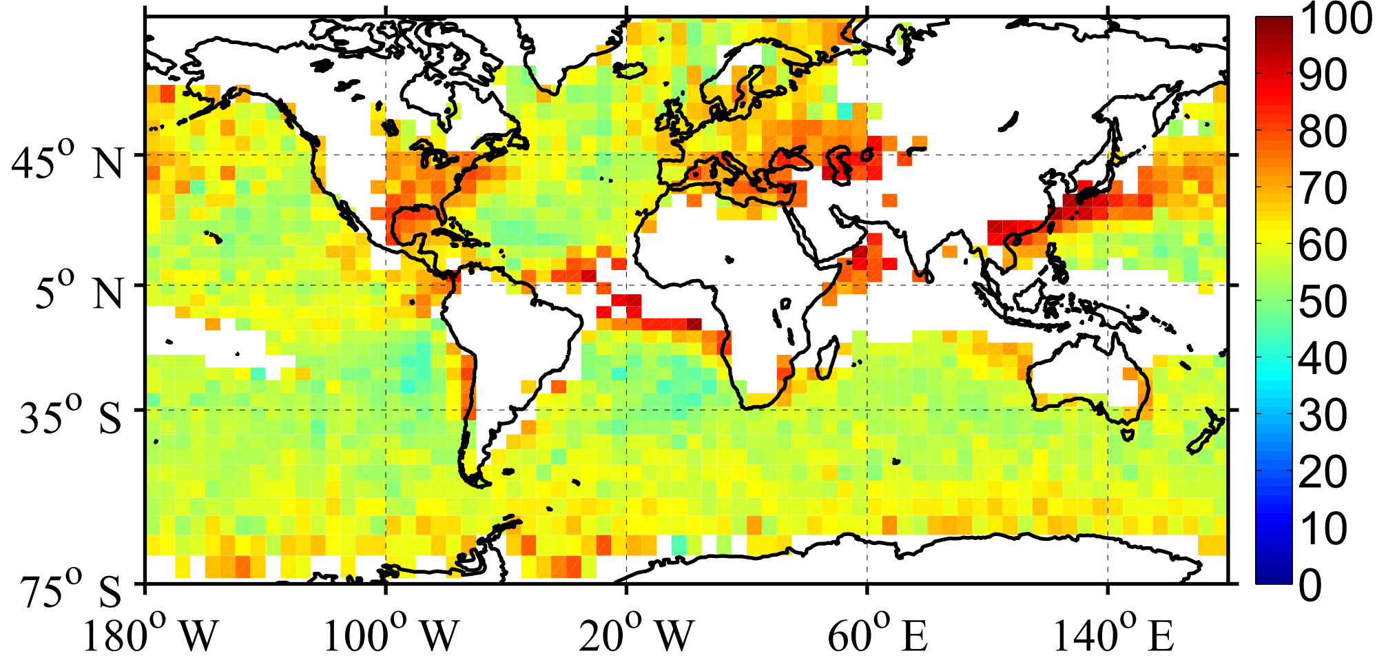
DJF max: 96 % median: 59 % mean: 59 %
