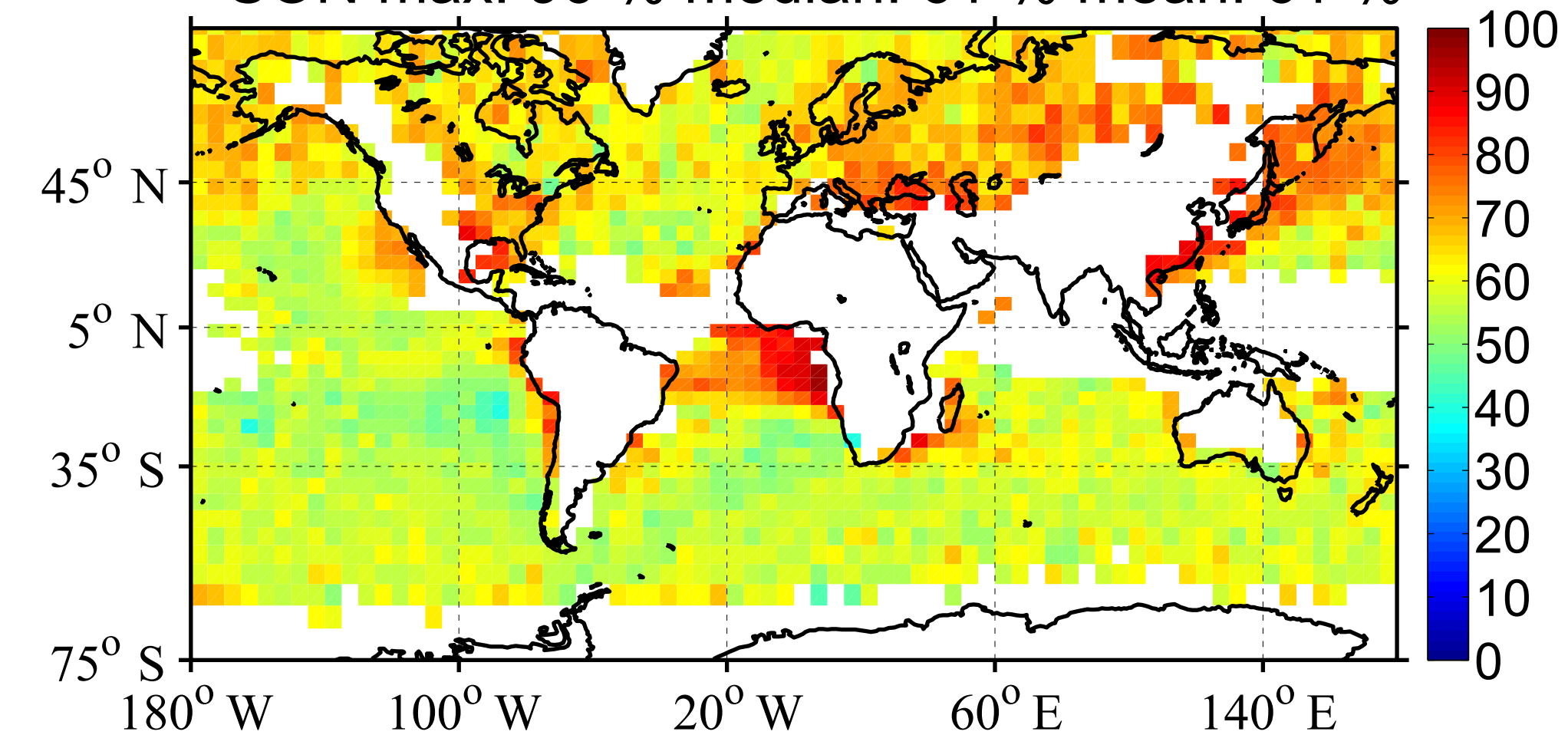
SON max: 96 % median: 61 % mean: 61 %
