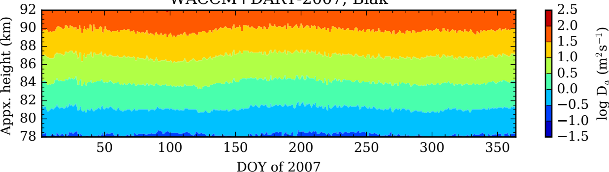
WACCM+DART-2007; Biak
