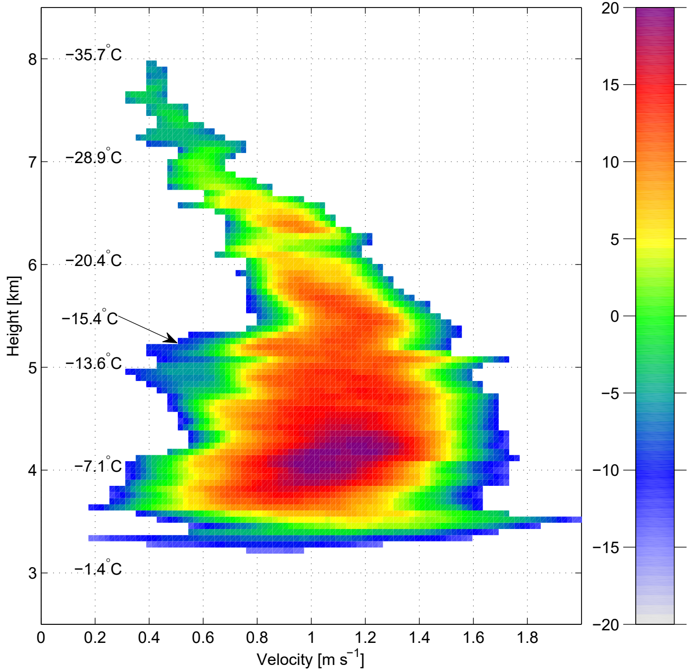
(a) 35 GHz spectral reflectivity [dBZ]
