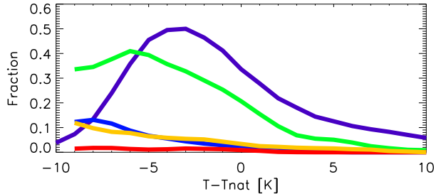
Ground-based lidar
