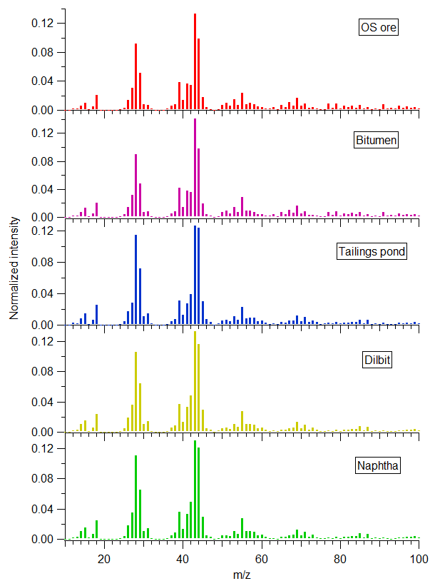
Figure S9. Representative AMS mass spectra for each OS-related oxidation experiment at OH exposure of \sim 1.5 \times 10^{12} \text{ molec cm}^{-3} \text{ s} .
