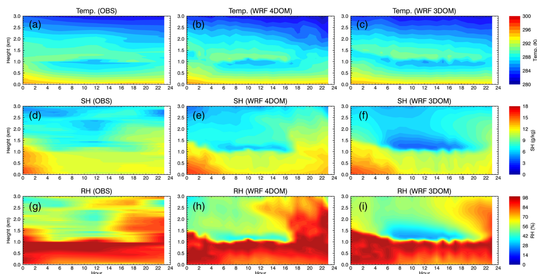
Figure 6. WRF-simulated and merged-sounding-observed (OBS) spatiotemporal evolutions of air temperature (Temp.), specific humidity (SH), and relative humidity (RH) for the high-altitude-plume case. Two sets of WRF simulations are presented here, one with four domains (the baseline configuration) and one with three domains (without the 19.2 km domain). The model results are averaged over 10 \times 10 grid points centering around the ENA ground site location from the innermost domain.
