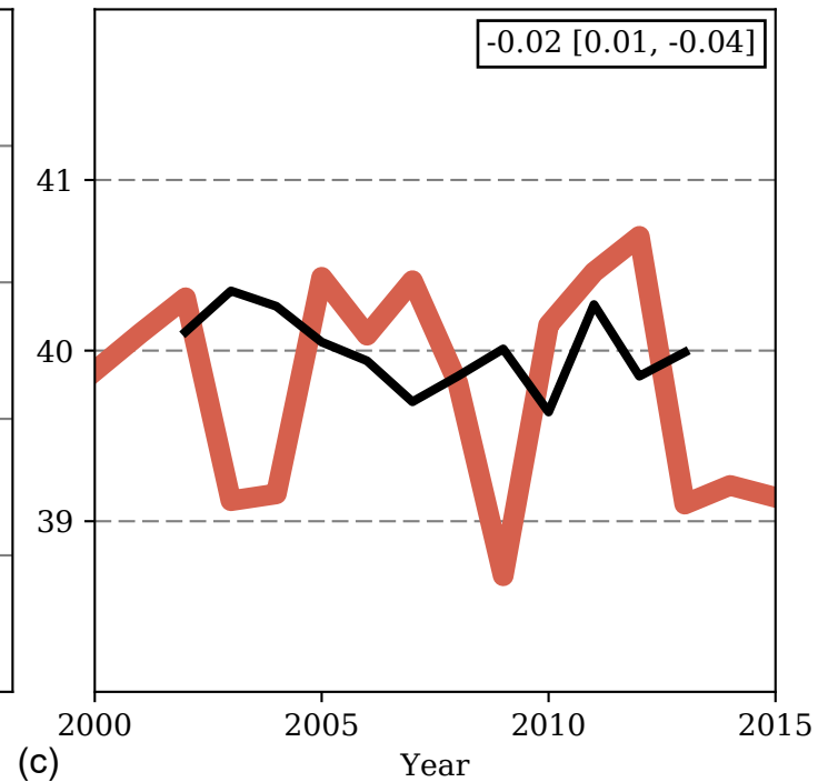
Pop. weighted MDA8 conc. [ppb]
