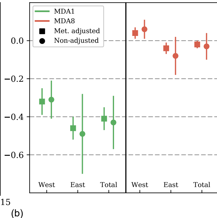
2000-2015 pop. weighted trends [ppb yr -1 ]
