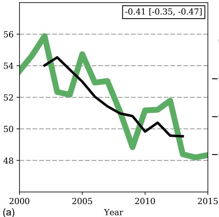
Pop. weighted MDA1 conc. [ppb]
