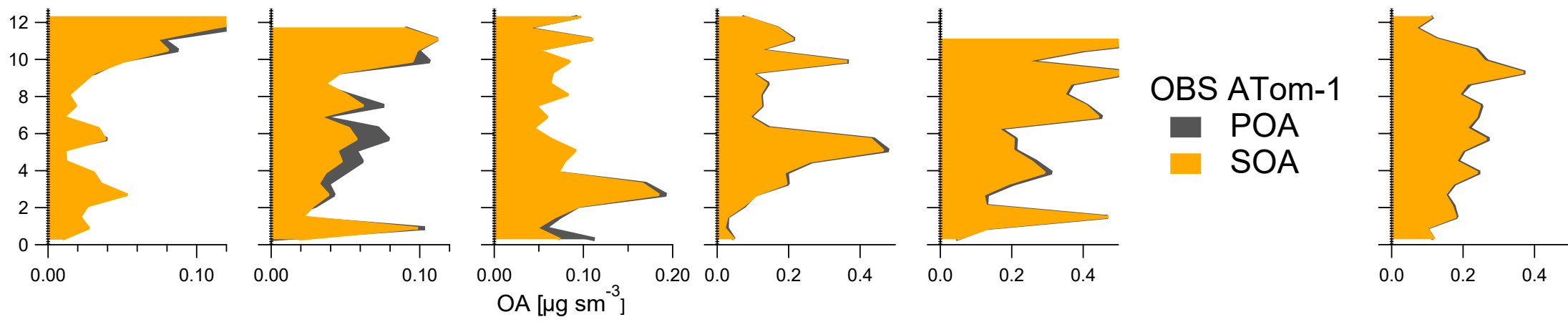
(b) ATom-1 OBS
