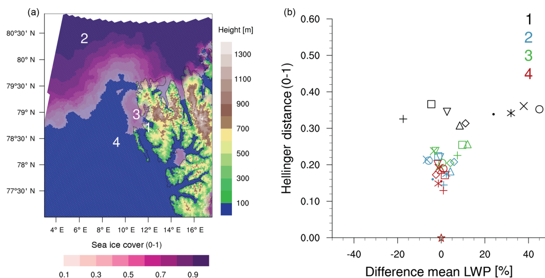
Figure 9. (a) Location of the four 10-grid-point subregions used for the representativity analysis: land (1), sea ice (2), mixed conditions (sea ice and open water, 3) and open water (4). (b) The Hellinger distance and differences in the mean LWP of the LWP PDFs of the surrounding grid points (different symbols) compared to the central point (star symbol) of the four subregions (overlaid). Values have been calculated for each day and then averaged over all 11 d.
