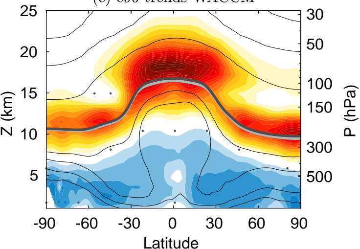
(c) e90 trends WACCM
