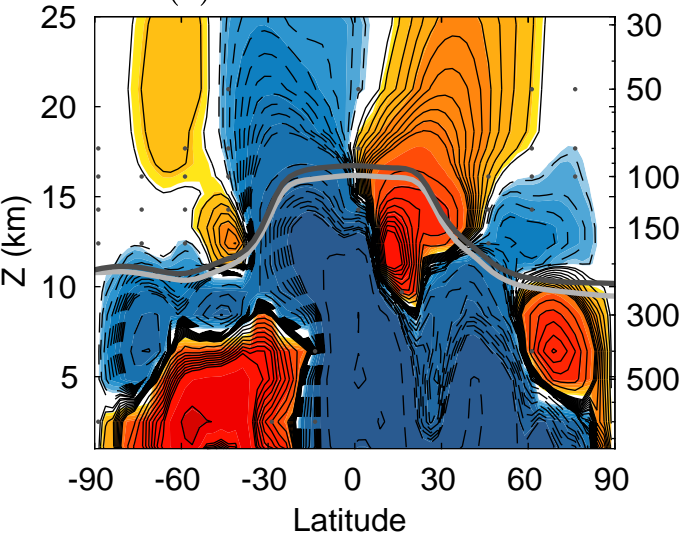
(c) \Psi^* trends EMAC-L47MA
