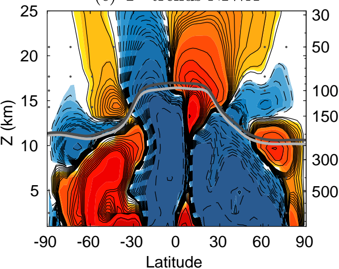
(e) \Psi^* trends NIWA
