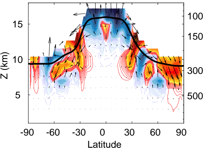
(c) st80 ADV trend GEOSCCM
