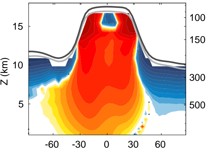
(c) st80 trends WACCM fODS
